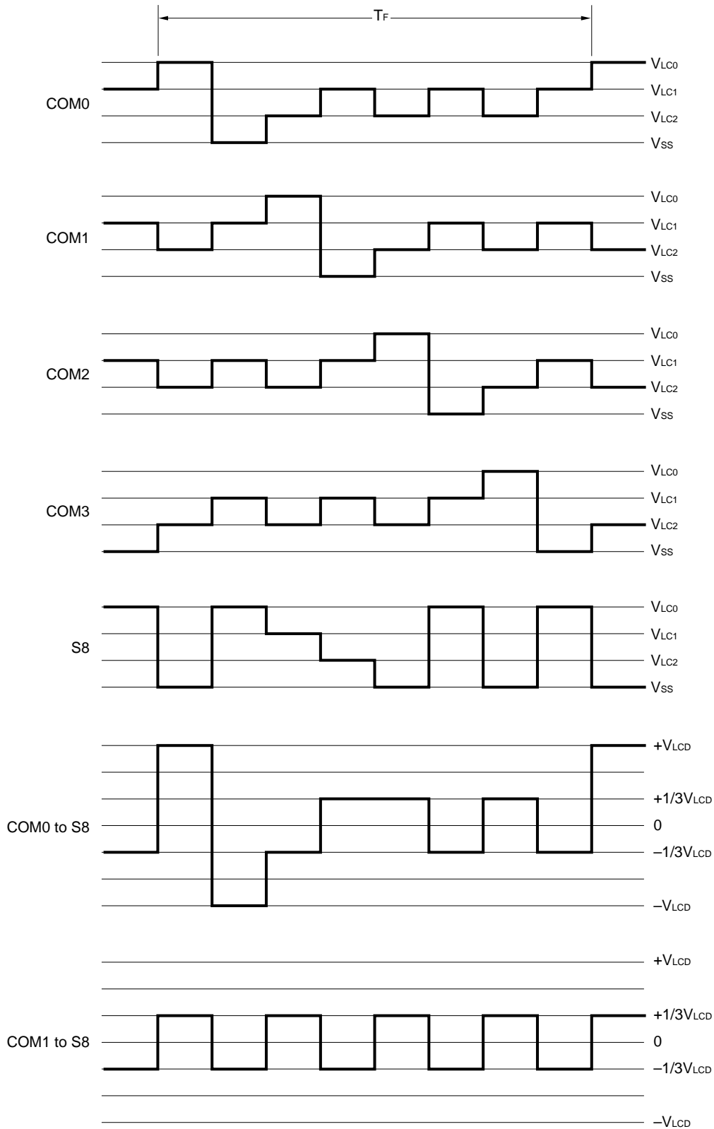
Figure 17-11: 4-Time-Division LCD Drive Waveform Examples (1/3 Bias Method)
