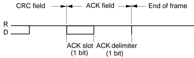
Figure 16-10: ACK Field
