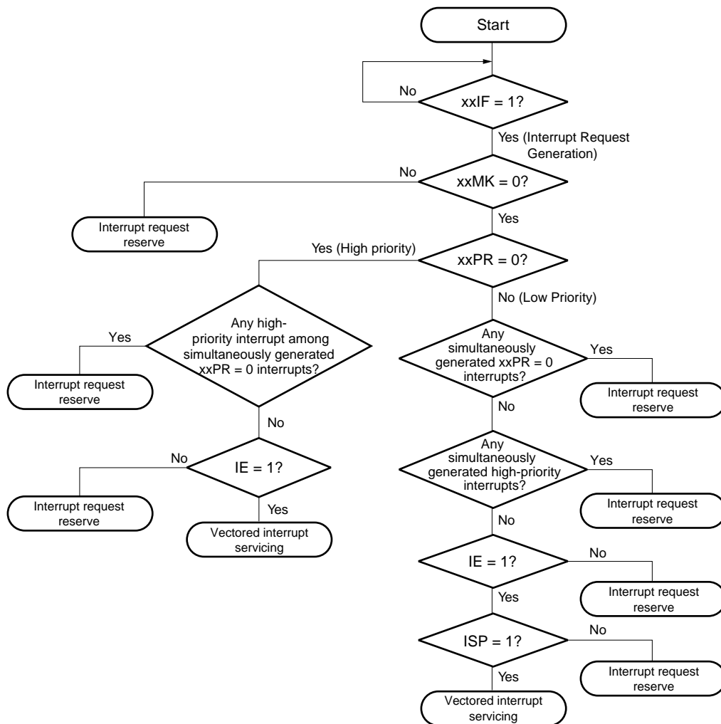
Figure 20-10: Interrupt Request Acknowledge Processing Algorithm
