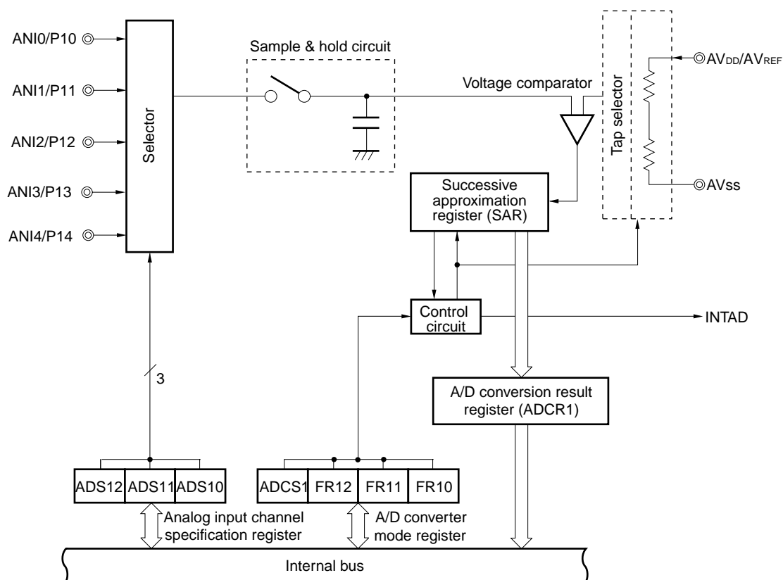
Figure 12-1: A/D Converter Block Diagram
