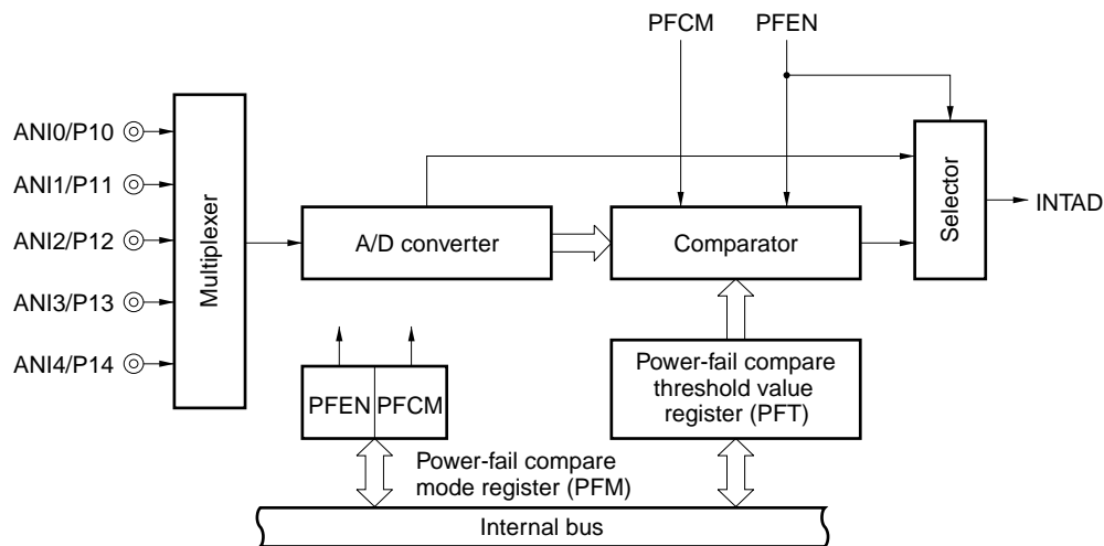
Figure 12-2: Power-Fail Detection Function Block Diagram
