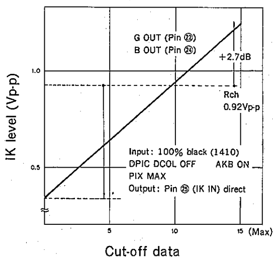
Cut-off control characteristics
