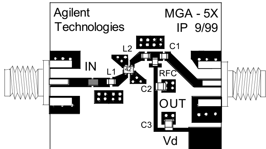
Figure 8. Complete 1.9 GHz Amplifier Circuit.
