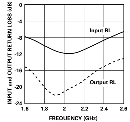
Figure 10. Input and Output Return Loss Results.
