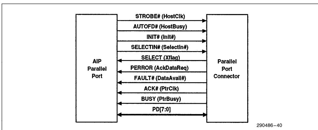
Figure 40. PS/2-Compatible Mode
