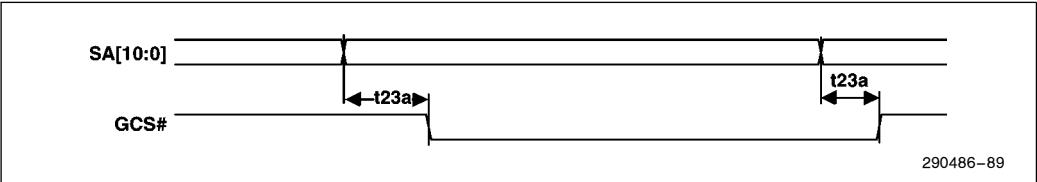
Figure 89. Game Port Timing
