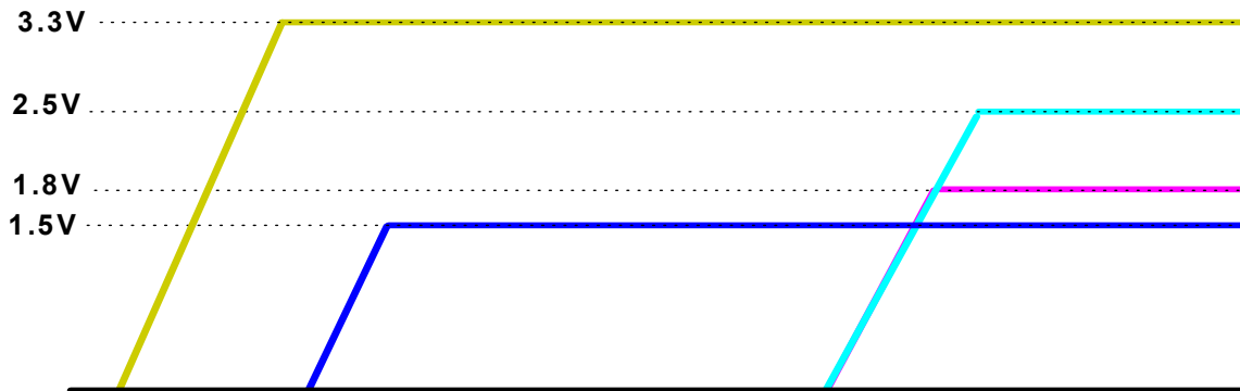
Figure 2A – Example Power Supply Sequencing and Tracking using the SMT4504. Any order of supply sequencing/tracking can be applied using the SMT4504.
