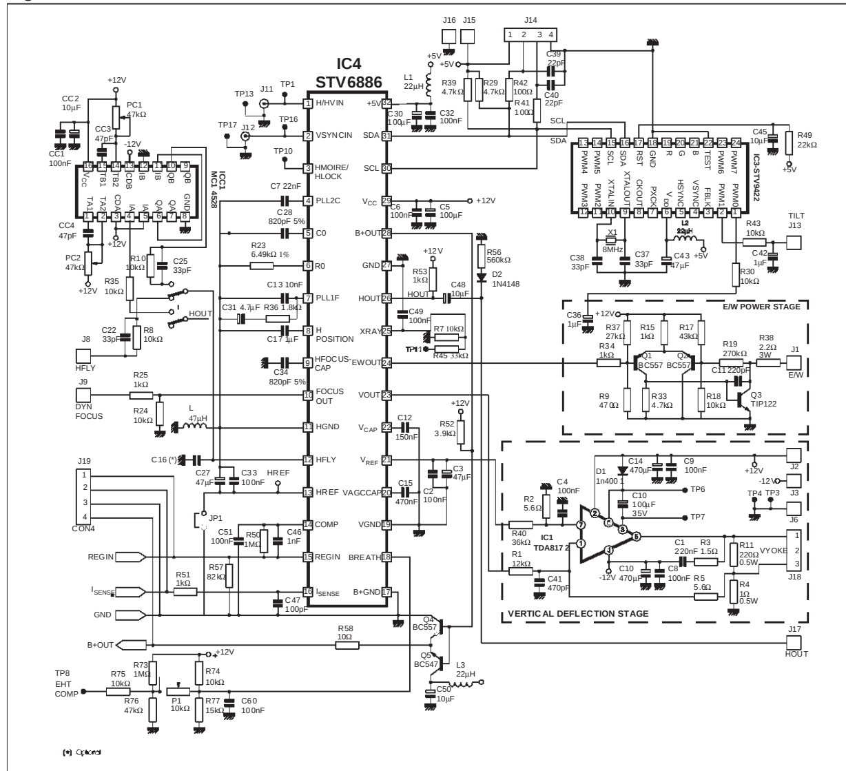
Figure 40. Demonstration Board
