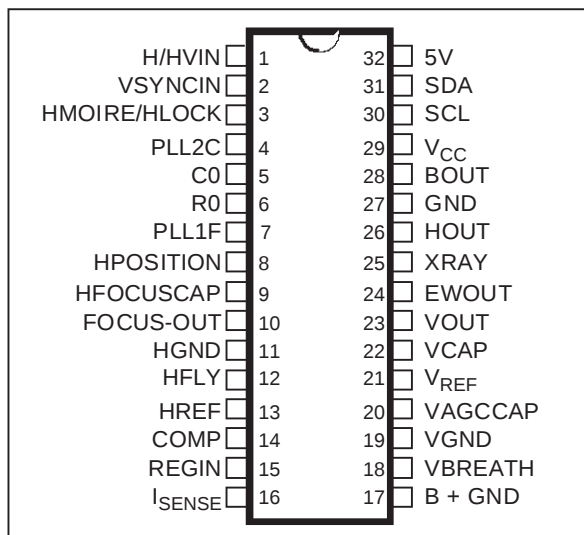
SHRINK32 (Plastic Package) ORDER CODE: STV6886
