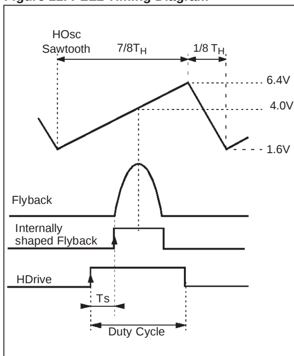
Figure 11. PLL2 Timing Diagram
