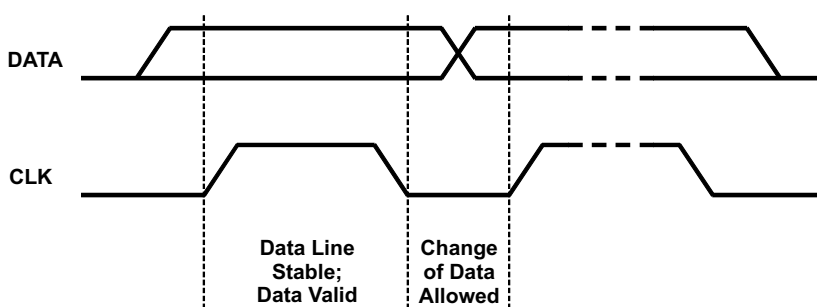
Figure 30. Bit Transfer on the Serial Interface
