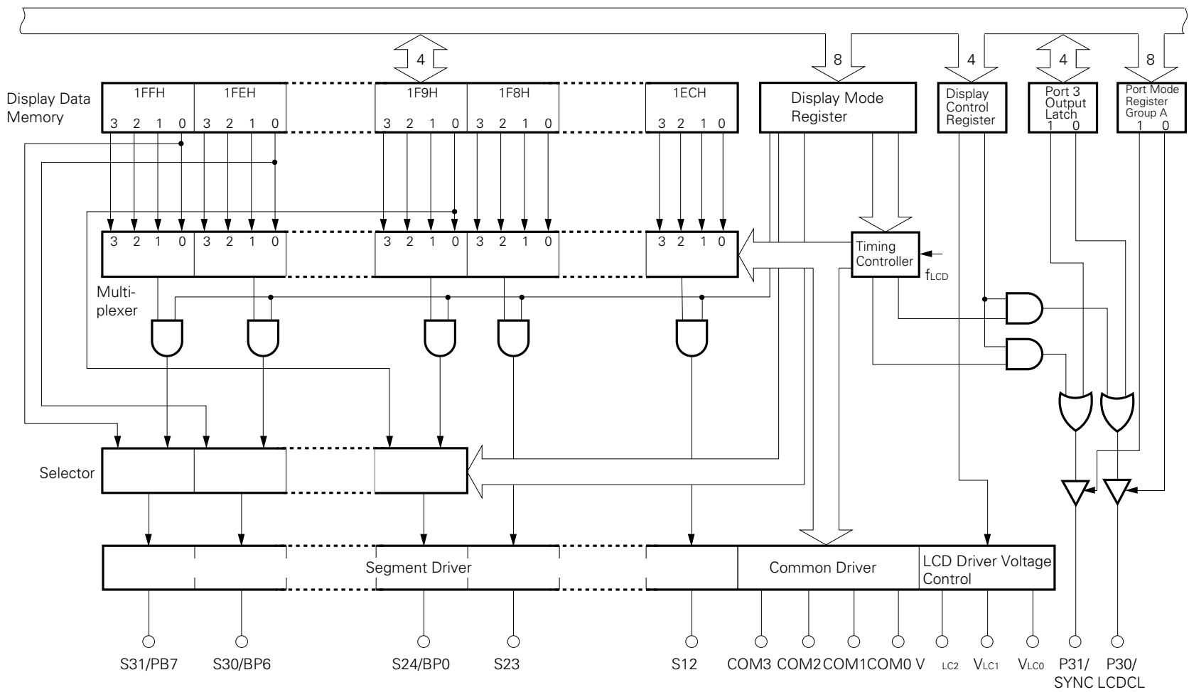
Fig. 5-7 LCD Controller/Driver Block Diagram
