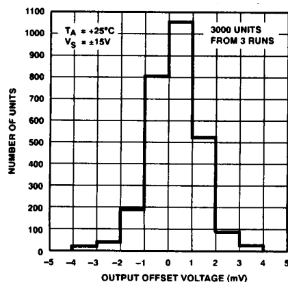
Figure 6. Typical Distribution of Output Offset Voltage
