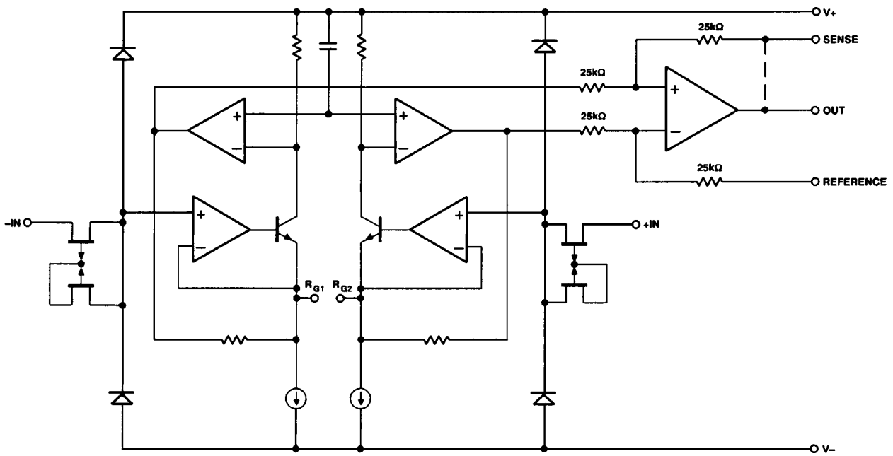
Figure 2. Simplified Schematic
