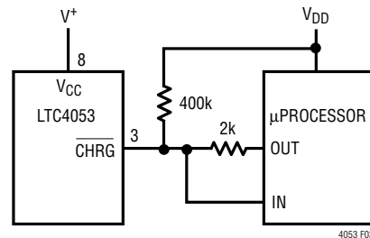
Figure 3. Microprocessor Interface
