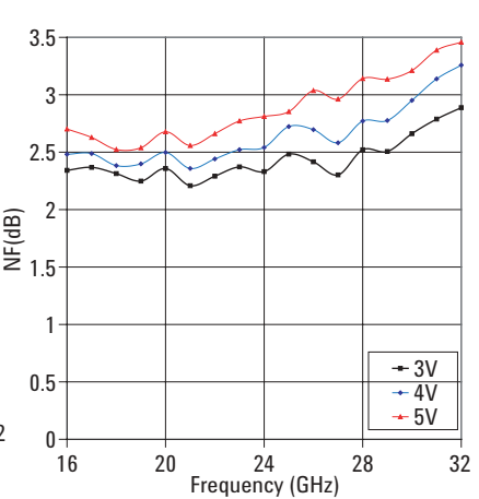
Figure 15: Noise Figure Over Vdd
