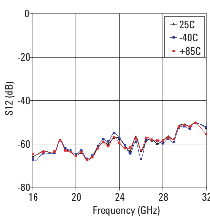
Figure 8. Isolation Over Temperature
