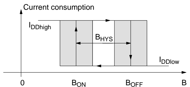
Fig. 4–6: Definition of magnetic switching points for the HAL584
