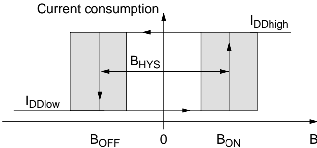
Fig. 1-3: Latching Sensor
