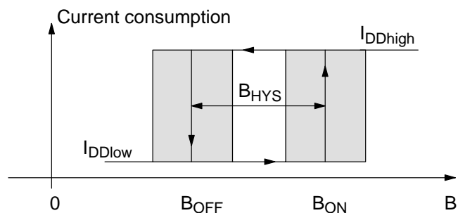
Fig. 4–2: Definition of magnetic switching points for the HAL573
