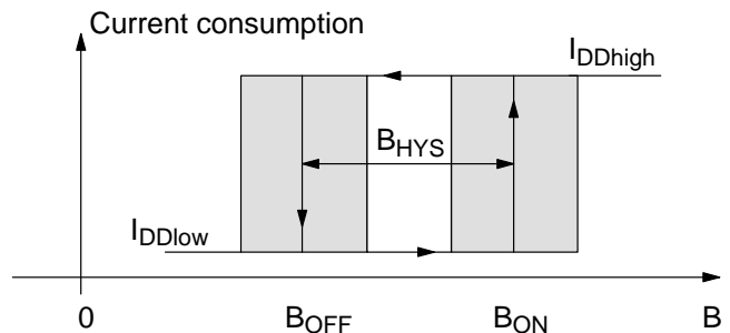
Fig. 4–1: Definition of magnetic switching points for the HAL571
