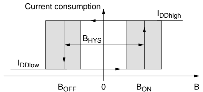
Fig. 4–4: Definition of magnetic switching points for the HAL575
