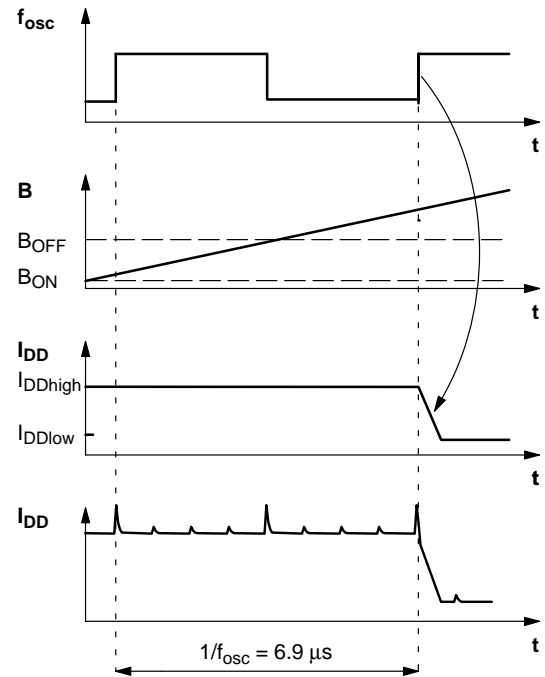
Fig. 2-2: Timing diagram (example: HAL581)
