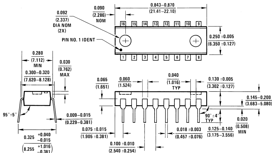
16-Lead Molded Dual-In-Line Package (N) Order Number LM614CN, LM614AIN, LM614BIN, LM614AMN or LM614MN NS Package Number N16A
