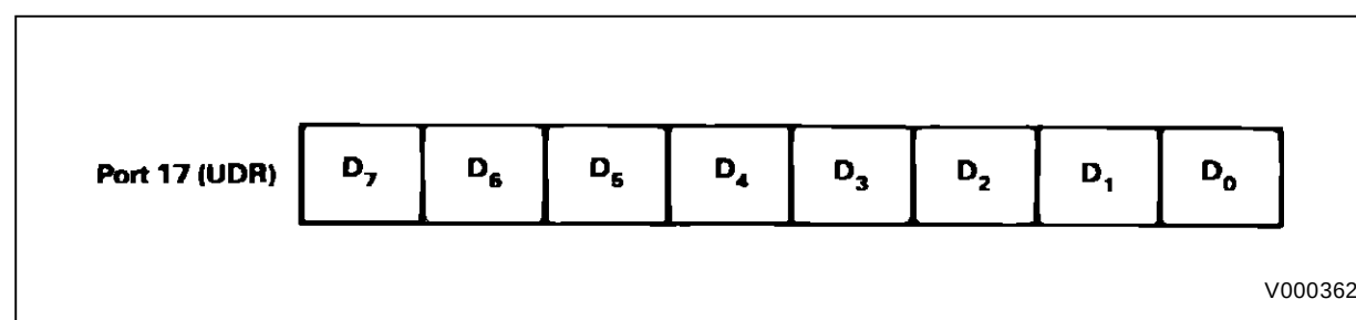
Figure 16 : USART Data Register.
