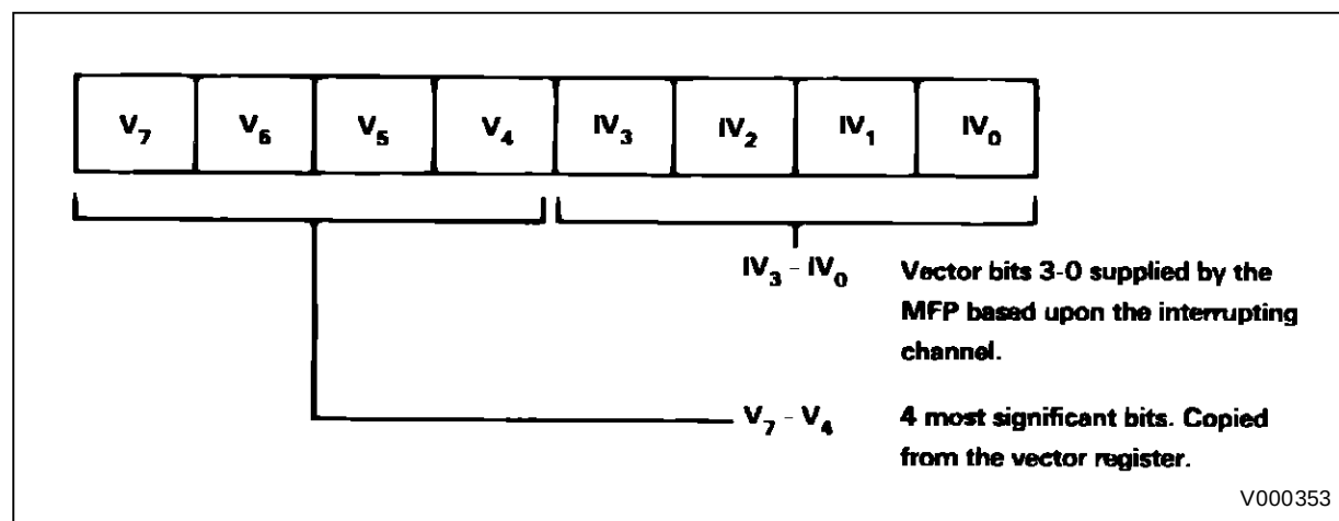
Figure 6 : Interrupt Vector.
