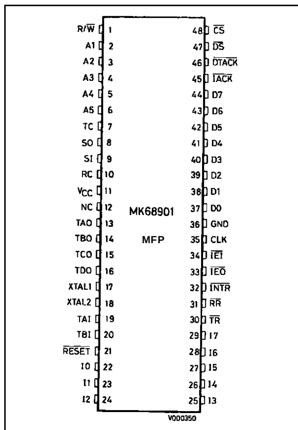
Figure 1 : Pin connections.
