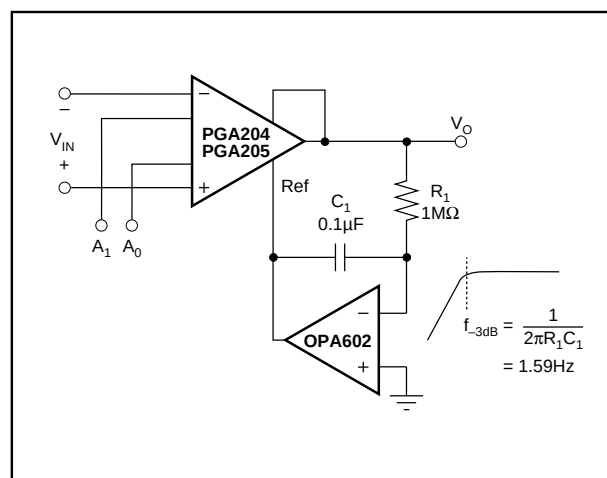
FIGURE 10. AC-Coupled PGIA.
