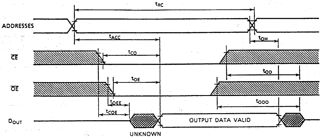
Read Cycle (1)
