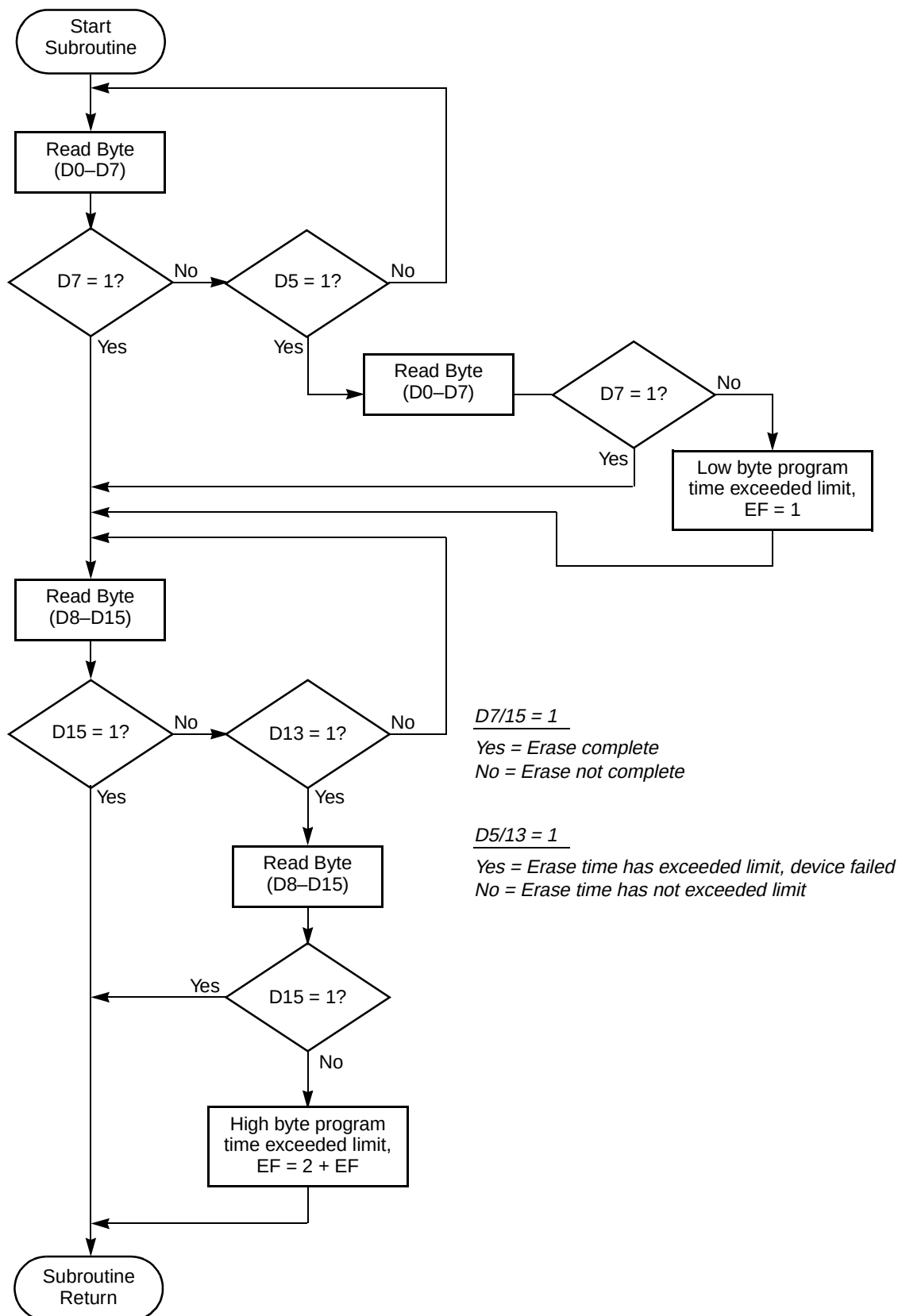
Figure 16. Word-Wide Software Polling Erase Subroutine
