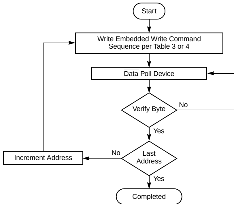
Figure 2. Embedded Programming Algorithm in Byte-Wide Mode
