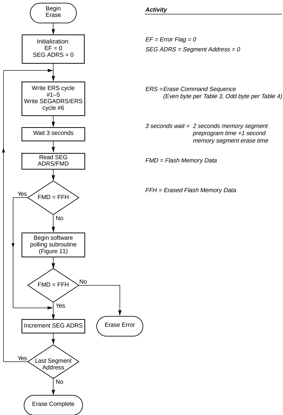
Figure 10. Byte-Wide Erasure Flow Chart
