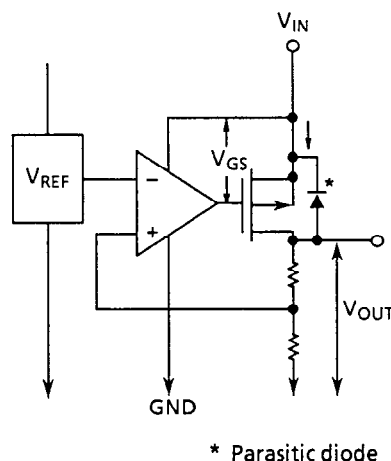
Figure 7 Control transistor
