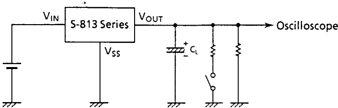
Figure 13 Measuring circuit
