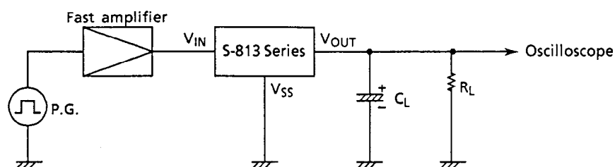
Figure 9 Measuring circuit
