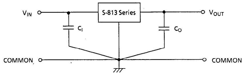
Figure 20 Standard circuit
