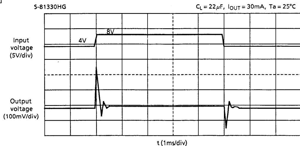
Figure 10 Type I ringing waveform
