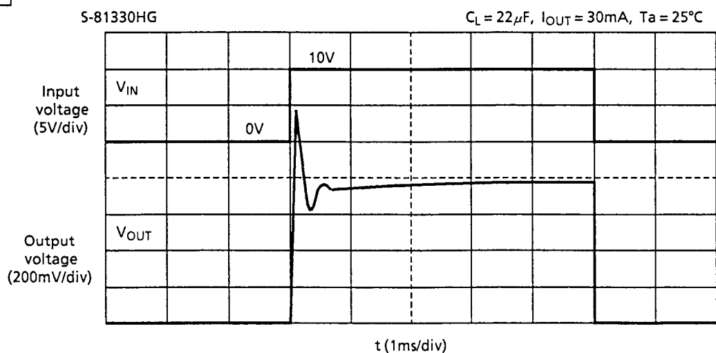
Figure 11 Type II ringing waveform
