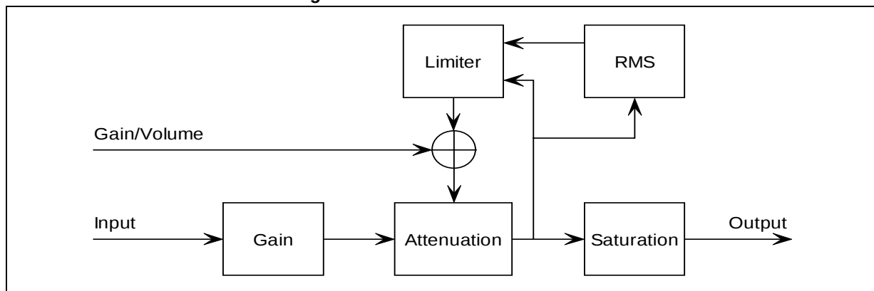
Basic Limiter and Volume Flow Diagram.
