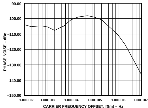
Figure 22. PLL Phase Noise L(F) vs. Frequency, V_{\text{POS}} = 3\text{ V} , C_3 = 0.1\text{ }\mu\text{F} , I_F = 10.7\text{ MHz}
