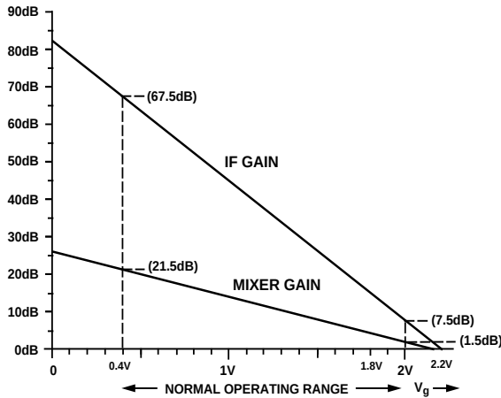
Figure 43. Gain Distribution for G_{REF} = 1.5 \text{ V}
