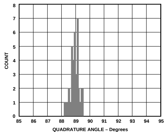
Figure 24. Demodulator Quadrature Angle, Histogram, T = +25^{\circ}\text{C} , V_{\text{POS}} = 3\text{ V} , I_F = 10.7\text{ MHz}
