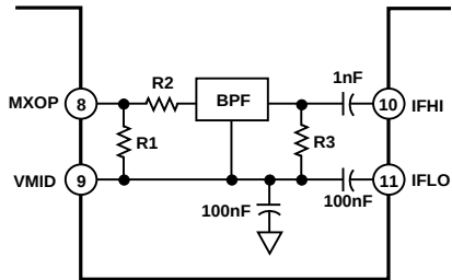
Figure 35. Suggested IF Filter Matching Network. The Values of R1 and R2 Are Selected to Keep the Impedance at Pin MXOP at 165 \Omega
