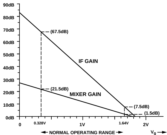
Figure 44. Gain Distribution for G_{REF} = 1.23 \text{ V}
