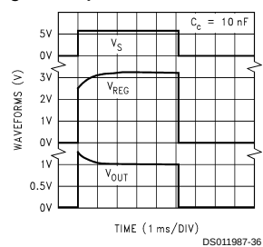
Response Time for 3.3V Version ( C_C = 10 nF )
