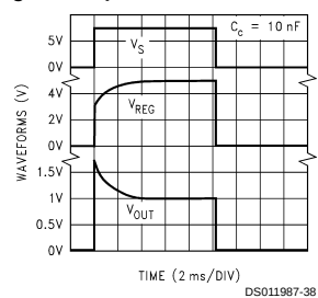
Response Time for 5V Version ( C_C = 10 nF )
