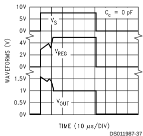
Response Time for 5V Version ( C_C = 0 pF )
