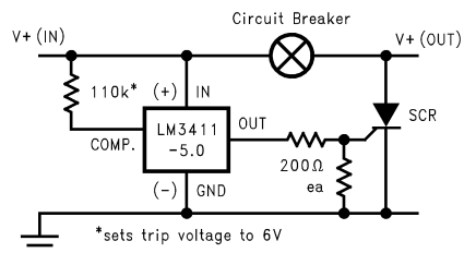
FIGURE 16. Overvoltage Crowbar
