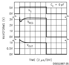
Response Time for 3.3V Version ( C_C = 0 pF )
