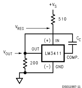
Circuit Used for Response Time
