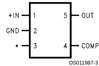
5-Lead Small Outline Package (M5)
