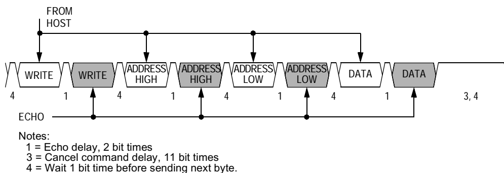
Figure 10-5. Write Transaction
