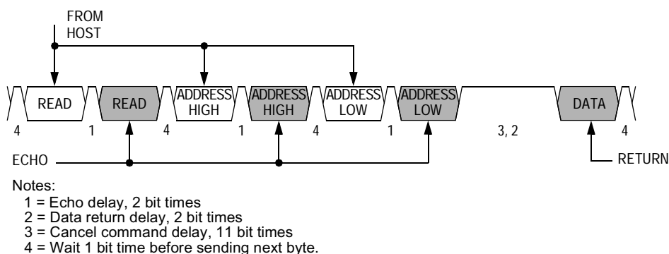
Figure 10-4. Read Transaction
