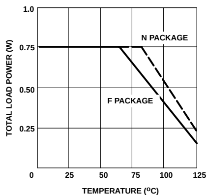
Total Load Power vs Temperature (NE590)
