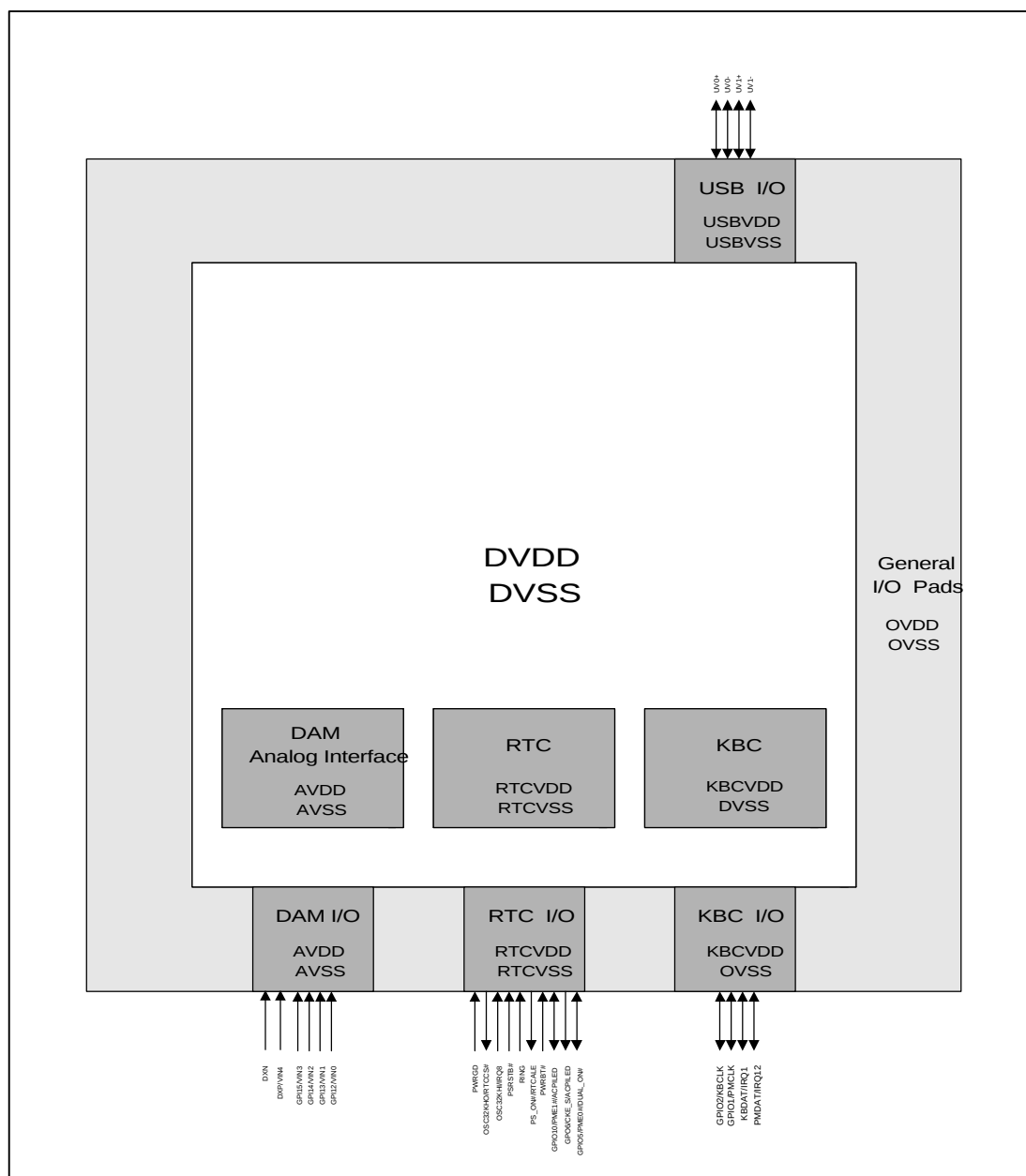
Figure 8.1-1 SiS5595 Internal Power Planes
