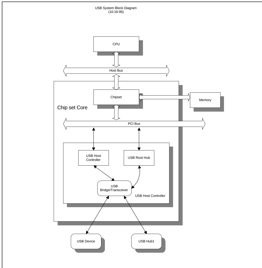
Figure 3.4-1 USB System Block Diagram
