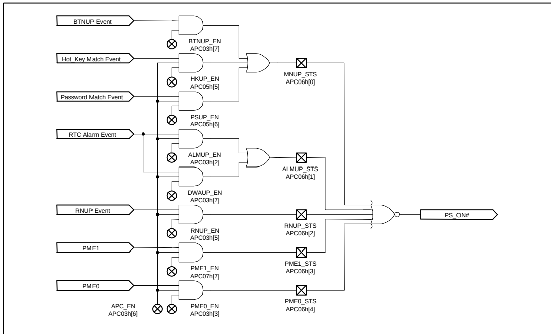
Figure 3.7-2 Power Up Request Events
