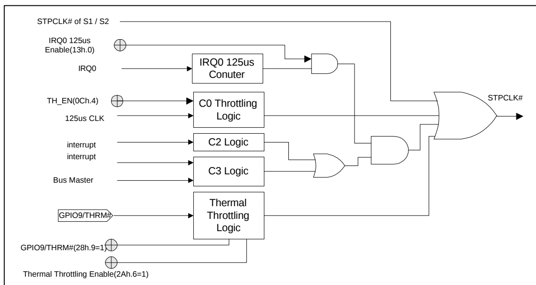
Figure 3.2-7 STPCLK# Source
