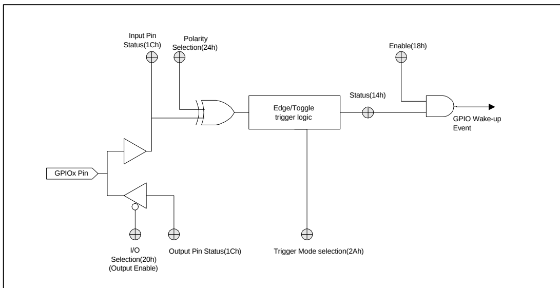
Figure 3.2-11 GPIO Logic
