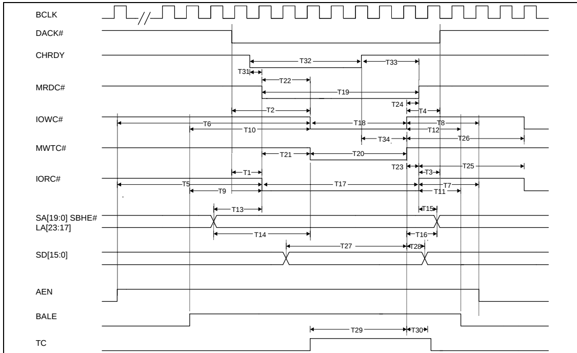
Figure 8.5-1 DMA Cycles
