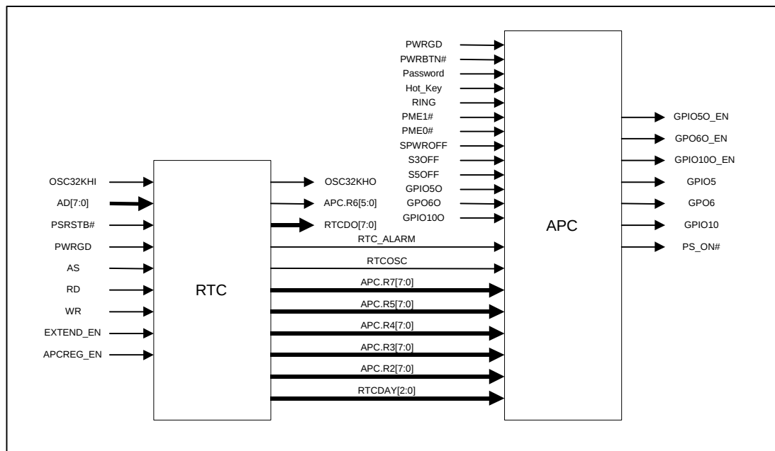
Figure 3.6-1 RTC Module Block Diagram
