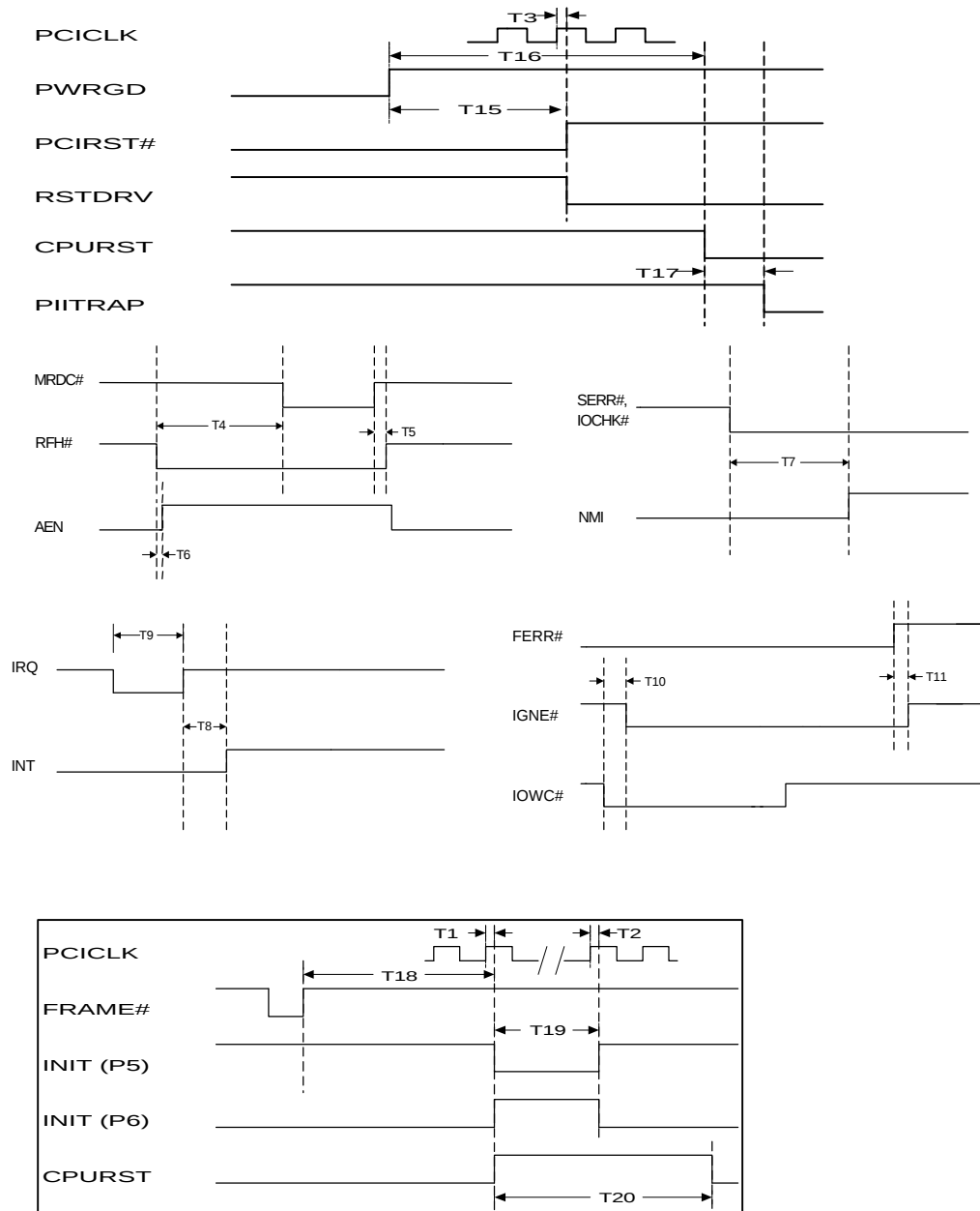
Figure 8.5-3 Miscellaneous Timing
