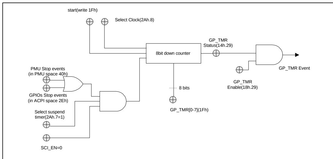
Figure 3.2-10 General Purpose Timer Logic
