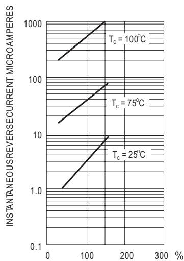
REVERSE VOLTAGE OF PERCENTAGE Fig.3- TYPICAL REVERSE CHARACTERISTIC
