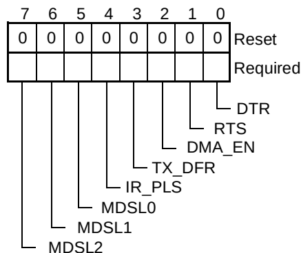
FIGURE 88. Modem Control Register, Extended Modes
