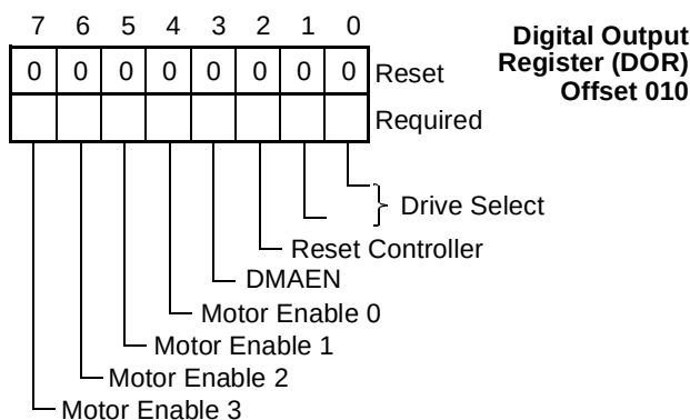
FIGURE 47. DOR Register Bitmap
