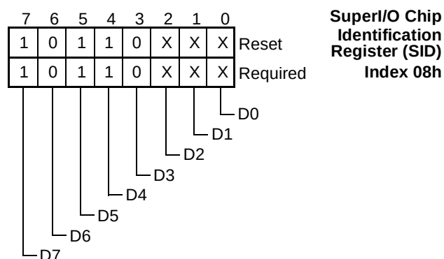
FIGURE 10. SID Register Bitmap
