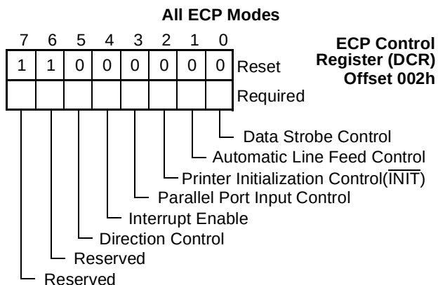
FIGURE 80. DCR Register Bitmap
