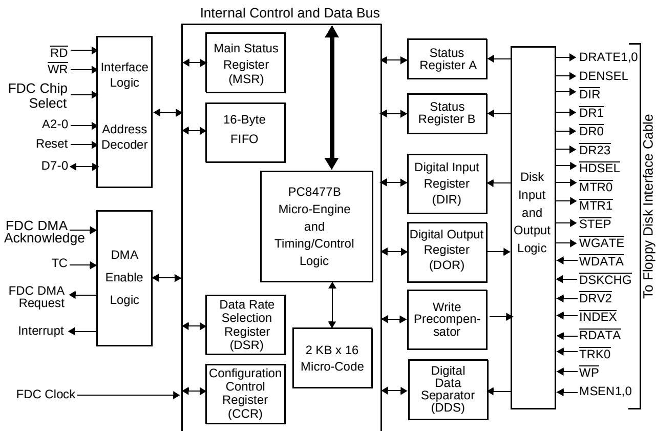
FIGURE 41. FDC Functional Block Diagram
