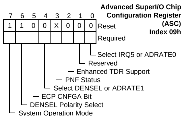
FIGURE 11. ASC Register Bitmap
