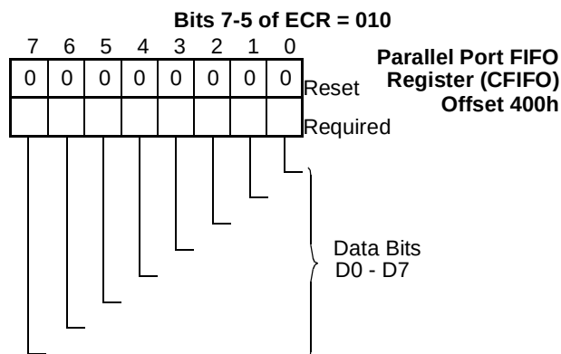
FIGURE 81. CFIFO Register Bitmap
