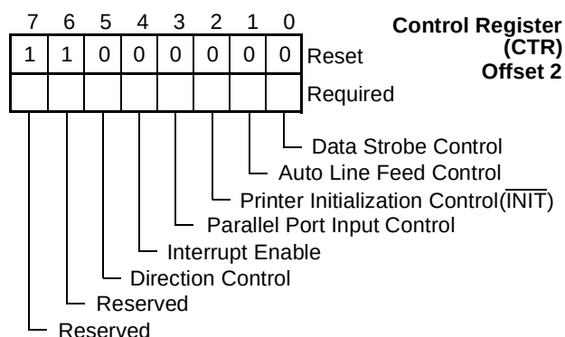
FIGURE 62. CTR Register Bitmap (SPP Mode) in PC87338
