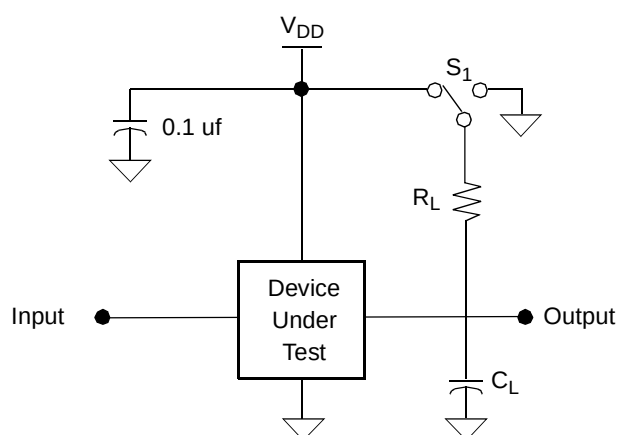
FIGURE 89. Load Circuit
