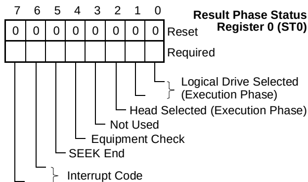
FIGURE 54. ST0 Result Phase Register Bitmap
