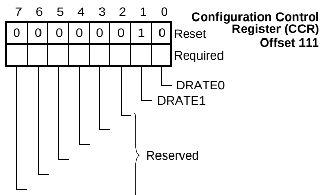
FIGURE 53. CCR Register Bitmap
