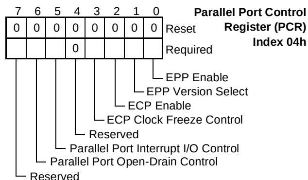
FIGURE 7. PCR Register Bitmap
