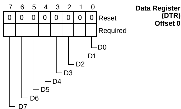
FIGURE 60. DTR Register Bitmap (SPP Mode)
