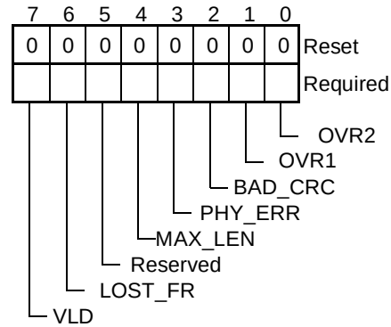
FIGURE 88. Frame Status Byte Register
