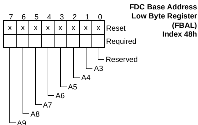
FIGURE 31. FBAL Register Bitmap
