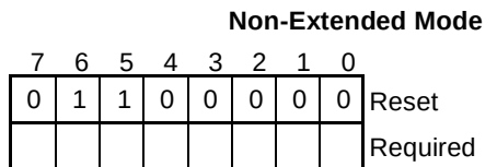
Link Status Register (LSR) Bank 0, Offset 05h
