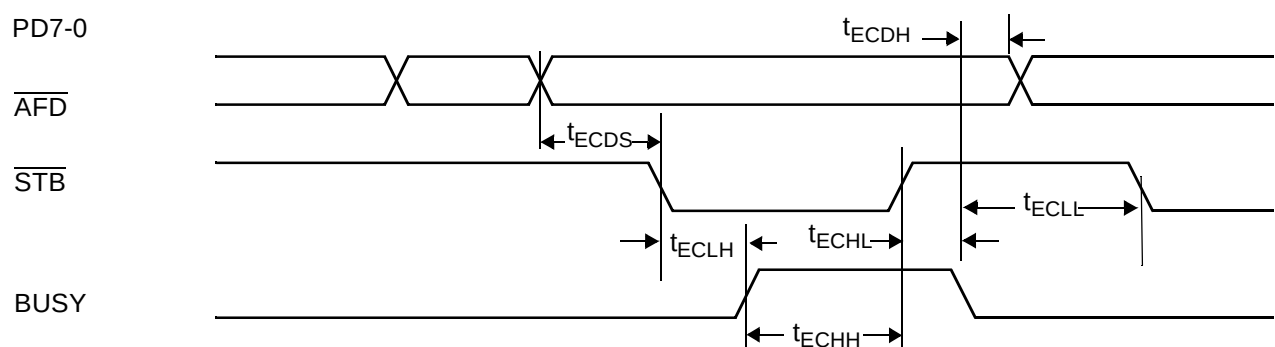
FIGURE 107. Parallel Port Forward Transfer Timing (ECP Mode)
