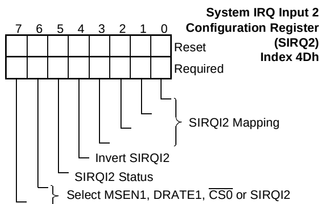
FIGURE 36. SIRQ2 Register Bitmap
