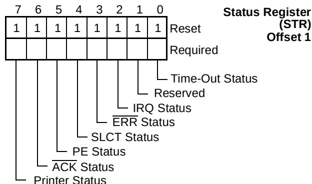
FIGURE 61. STR Register Bitmap (SPP Mode)
