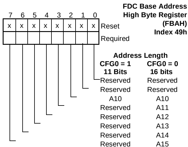
FIGURE 32. FBAH Register Bitmap
