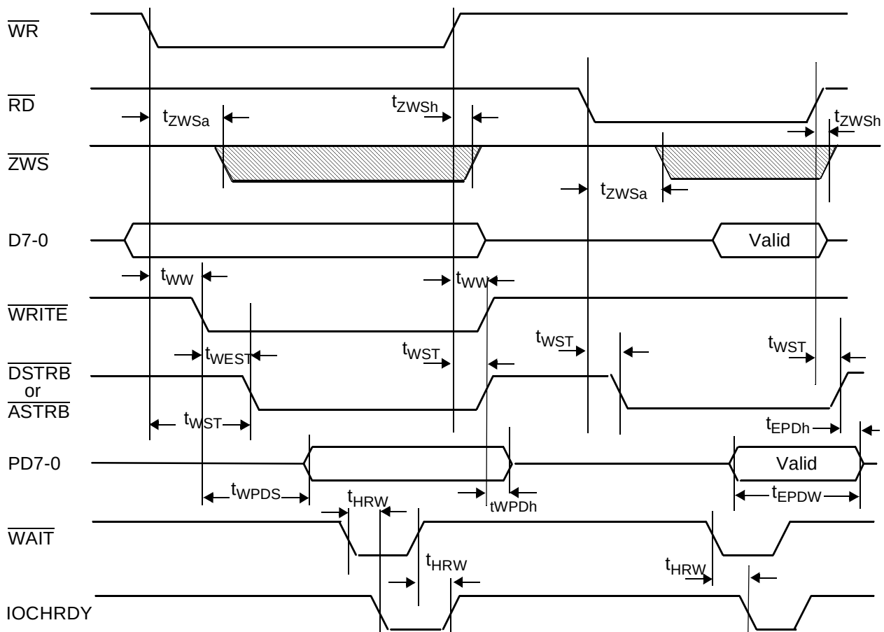
FIGURE 105. Parallel Port Data Transfer Timing (EPP 1.7 Mode)
