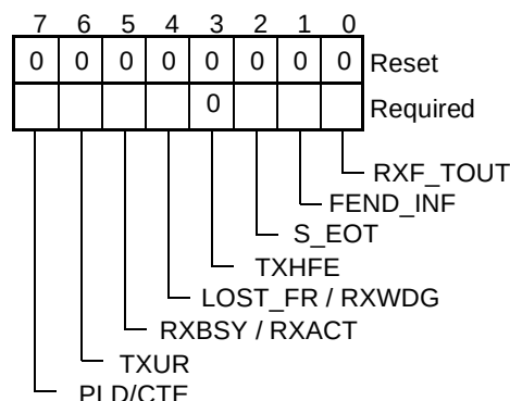
FIGURE 88. Auxillary Status and Control Register
