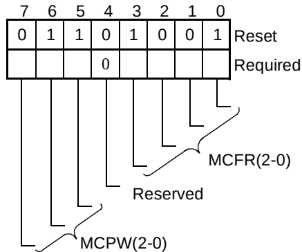
FIGURE 88. Infrared Transmitter Modulator Control Register
