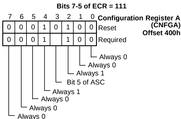
FIGURE 84. CNFGA Register Bitmap
