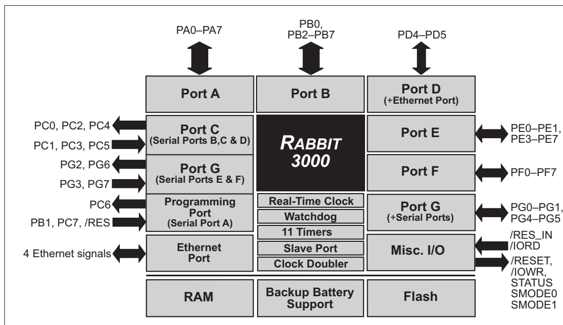
Figure 3. Use of Rabbit 3000 Ports
