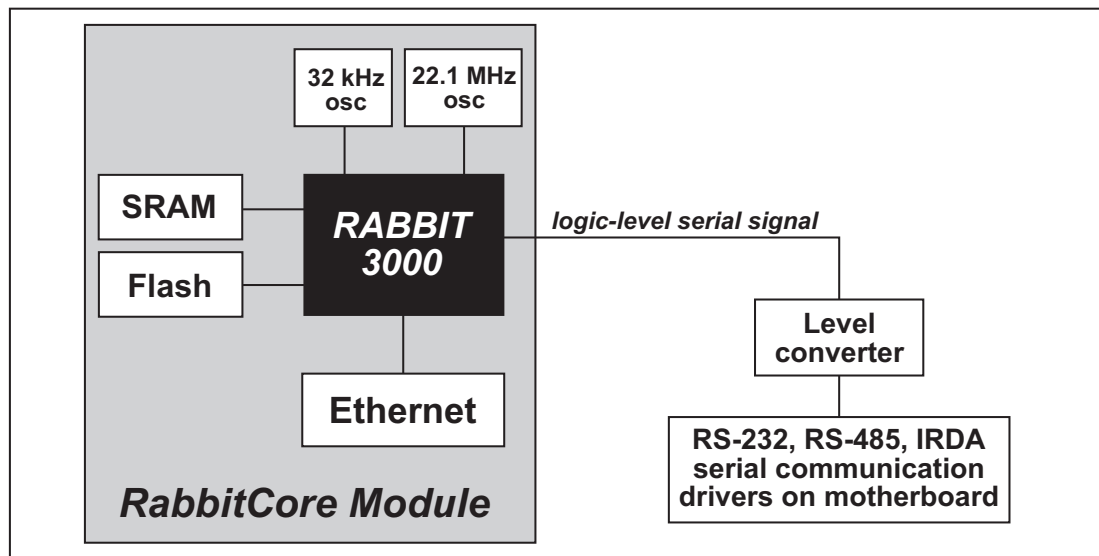
Figure 1. RCM3200 Subsystems
