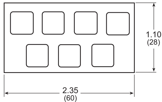
Figure C-3. Keypad Template
