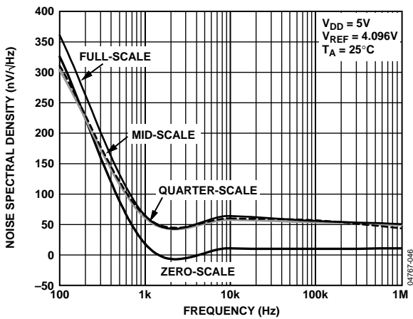
Figure 30. Noise Spectral Density
