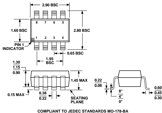
Figure 53. 8-Lead Small Outline Transistor Package [SOT-23] (RJ-8) Dimensions shown in millimeters
