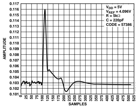
Figure 24. AD5060 Digital-to-Analog Glitch Energy
