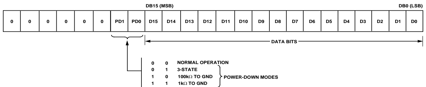
Figure 41. AD5060 Input Register Content
