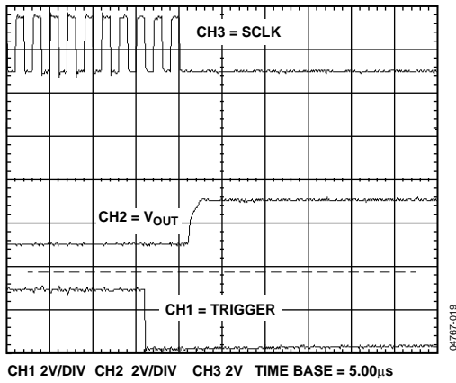
Figure 29. Time to Exit Power-Down to Midscale
