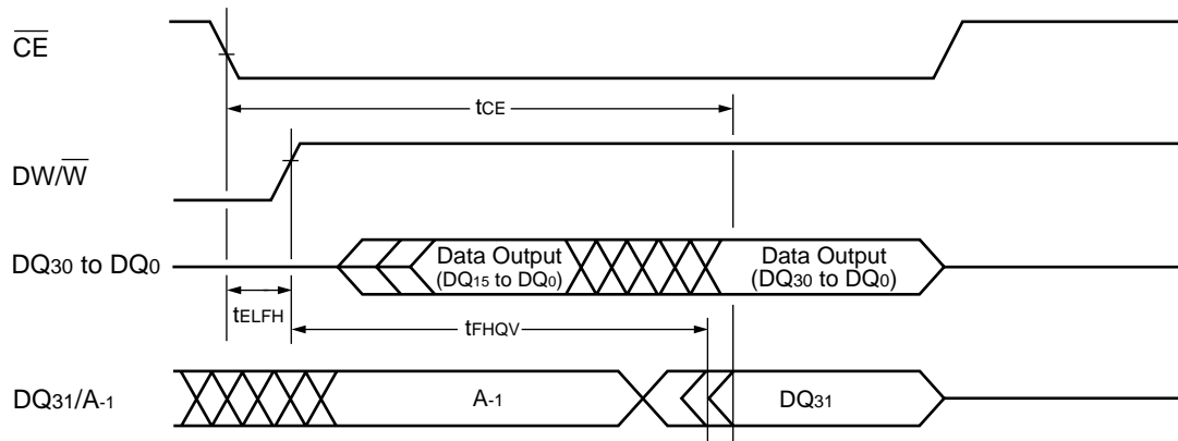
Figure 12 Double Word Mode Configuration Timing Diagram
