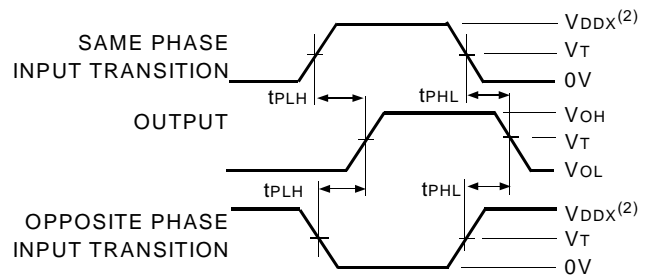
Propagation Delay
