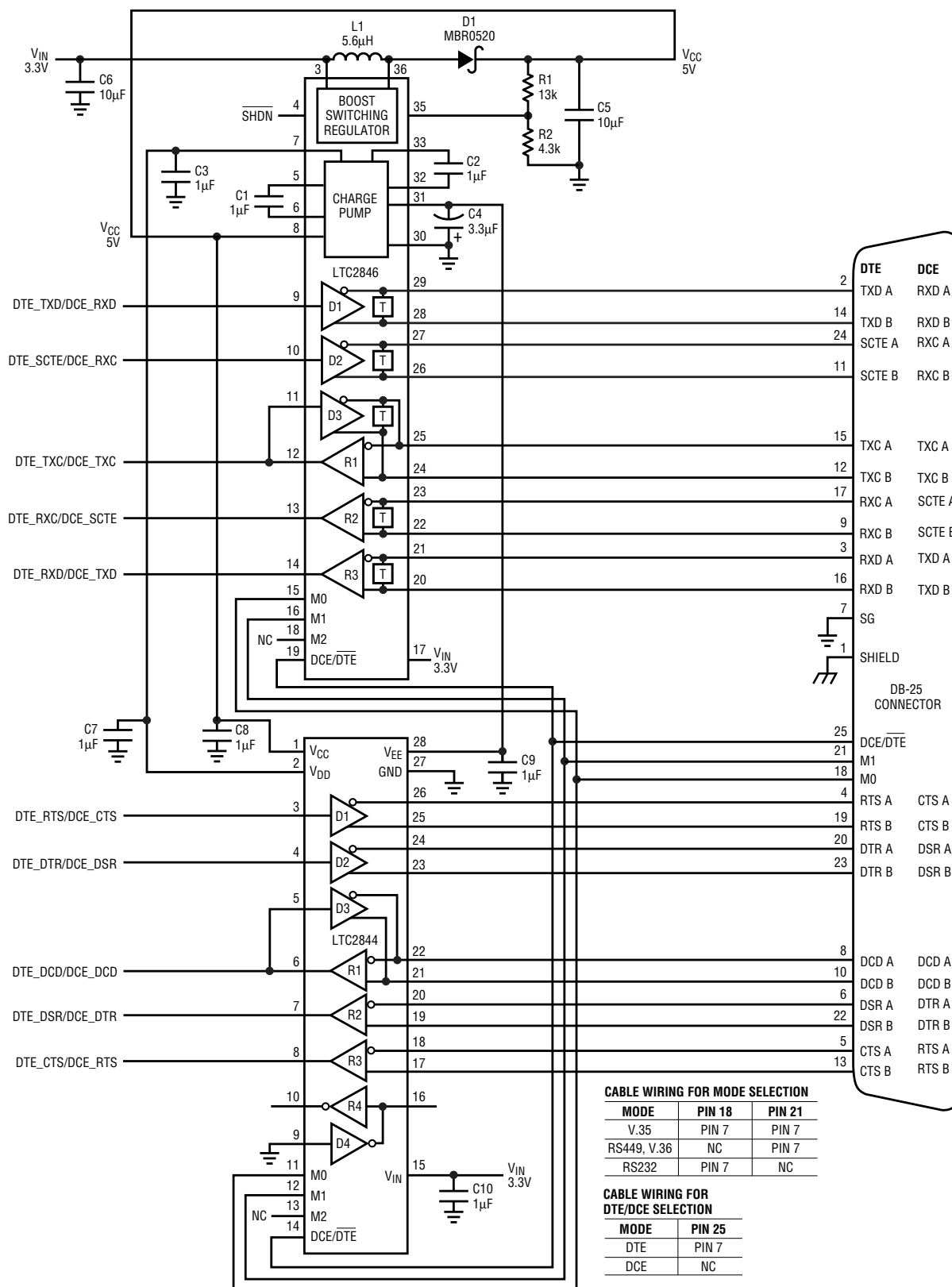
Figure 27. Cable-Selectable Multiprotocol DTE/DCE Port with DB-25 Connector
