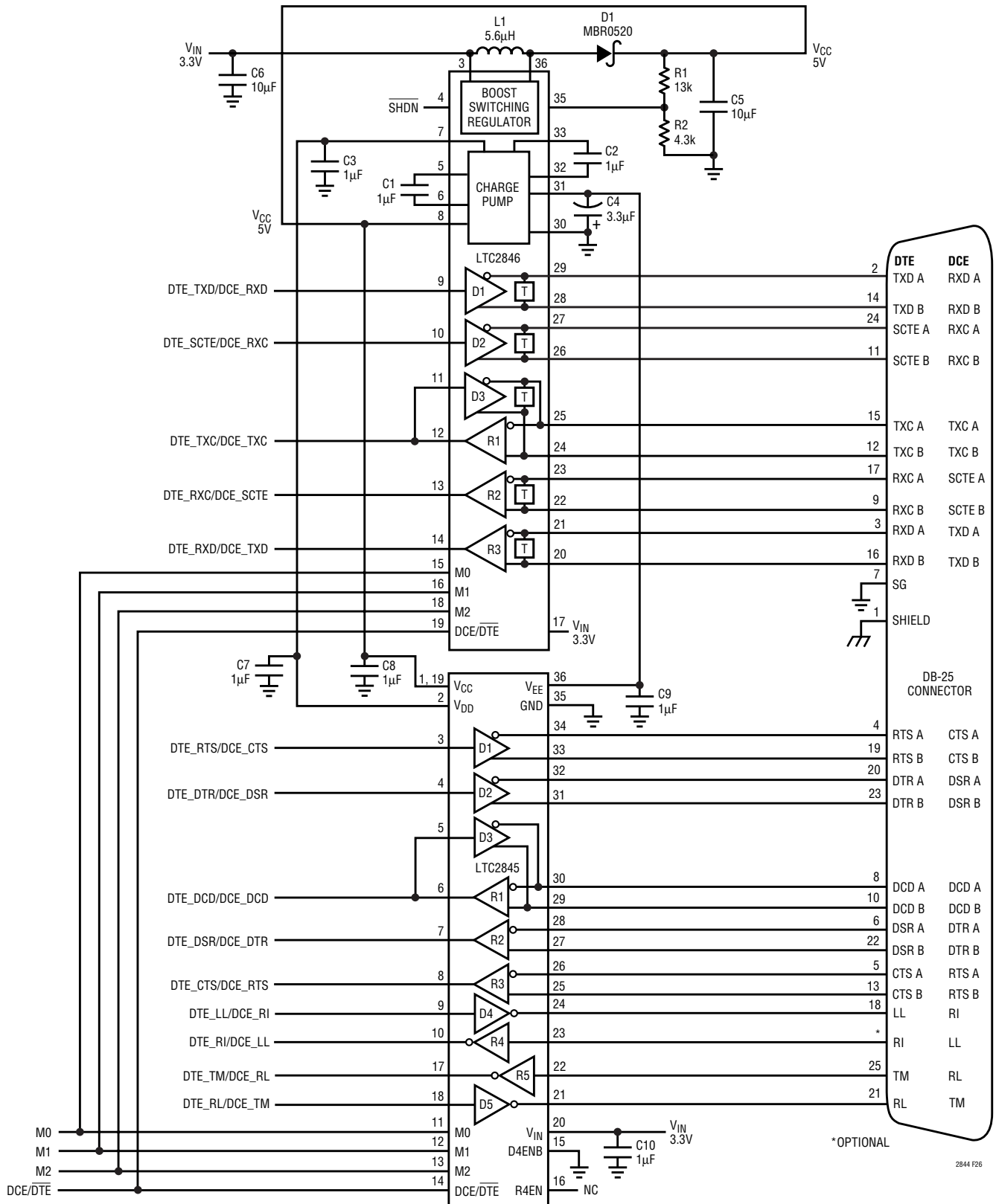
Figure 26. Controller-Selectable Multiprotocol DTE/DCE Port with RL, LL, TM and DB-25 Connector
