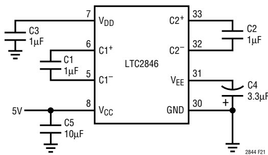
Figure 21. Charge Pump
