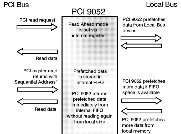
Figure 3-2. PCI 9052 Read Ahead Mode
