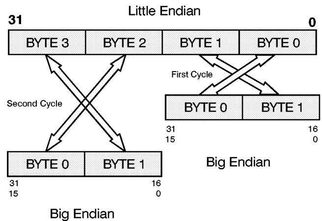
Figure 2-4. Big/Little Endian—16 Bit Local Bus
