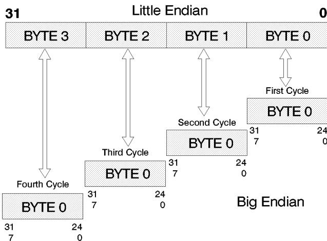
Figure 2-5. Big/Little Endian—8 Bit Local Bus
