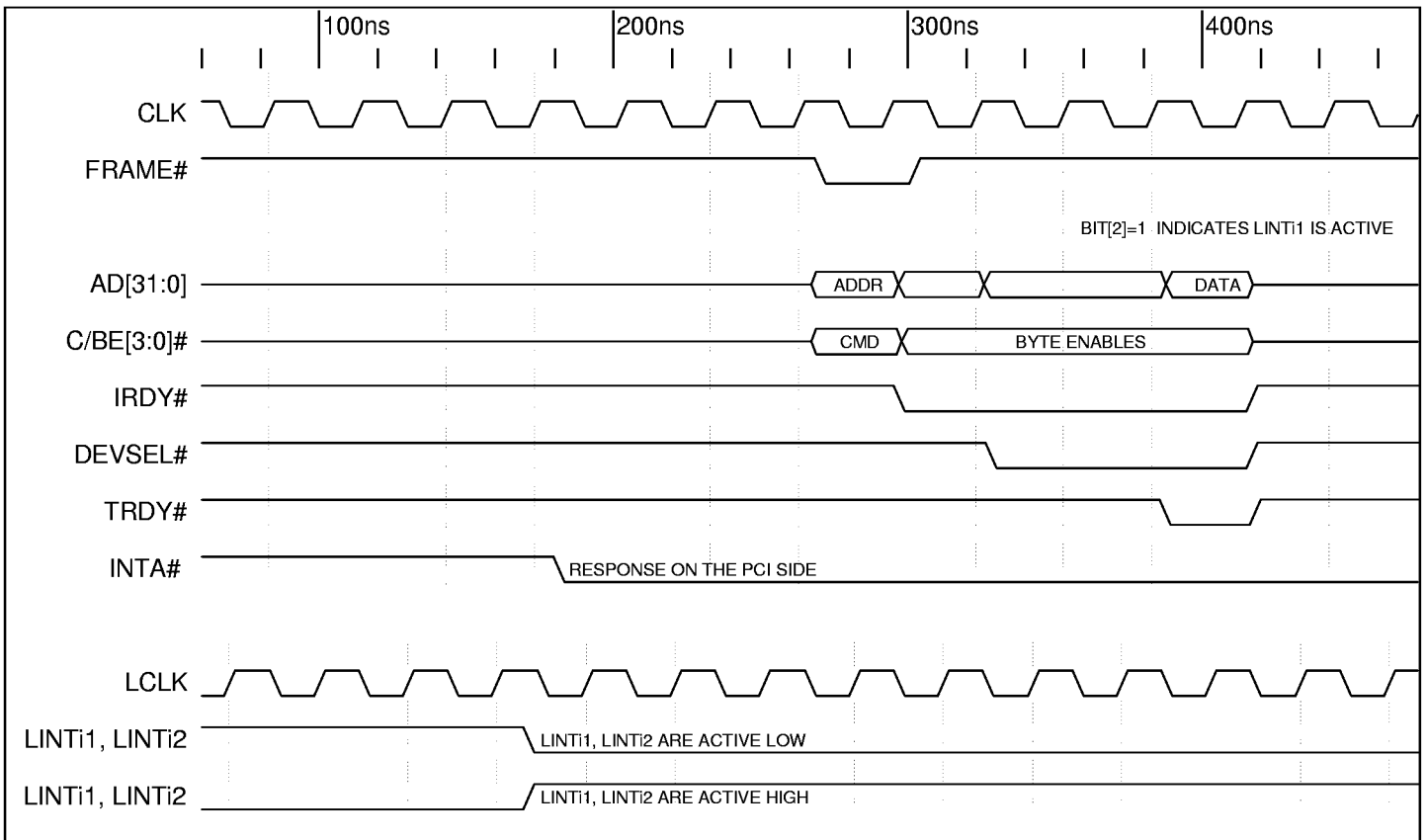
Timing Diagram 9-3. Local LINTi# Input Asserting PCI Output INTA#
