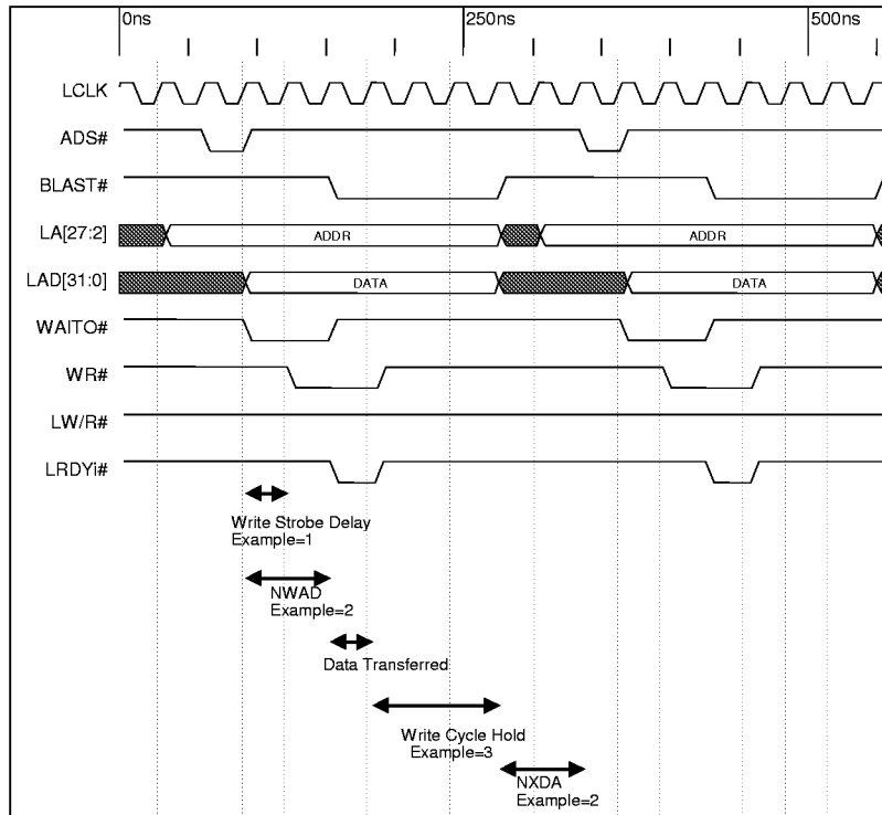
Figure 2-1. PCI 9052 Single Cycle Write
