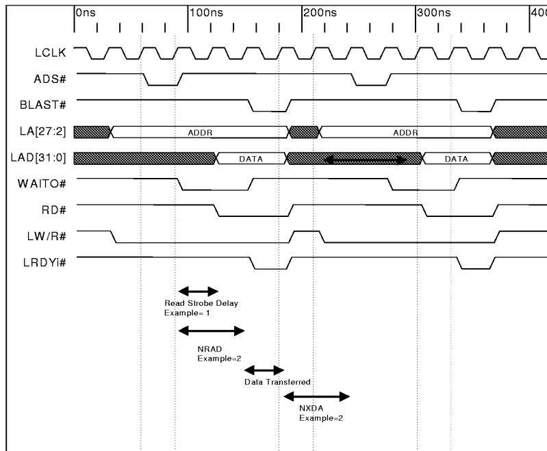
Figure 2-2. PCI 9052 Single Cycle Read
