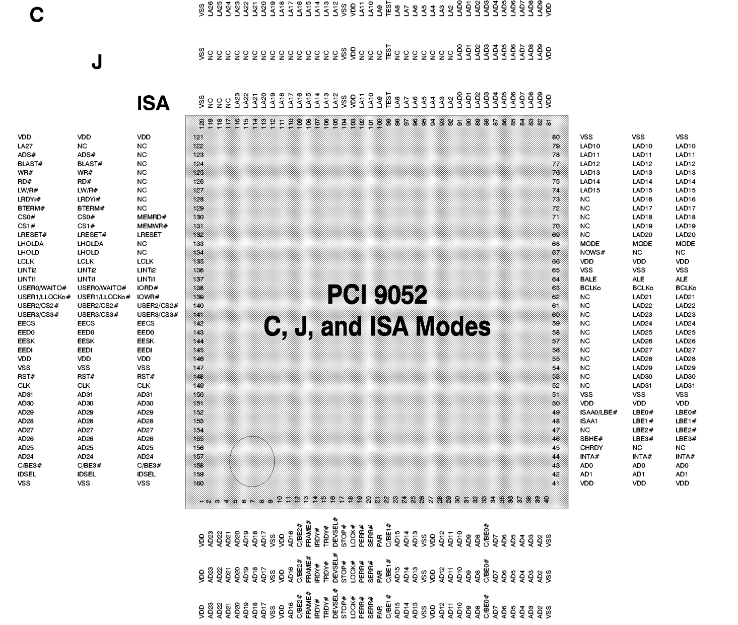
Figure 8-3. PCI 9052 Pin Out (C, J, and ISA Modes)
