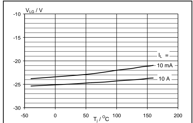
Fig.25. Typical negative load clamping voltage. V_{LG} = f(T_j) ; parameter I_L ; condition V_{IG} = 0\text{V}
