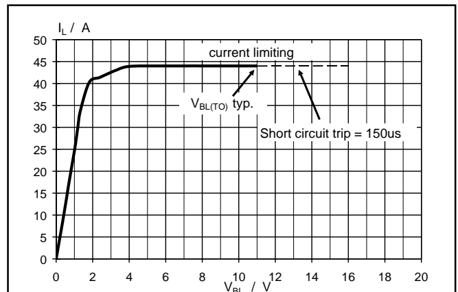
Fig.27. Typical overload characteristic, T_{mb} = 25\text{ }^{\circ}\text{C} . I_L = f(V_{BL}) ; condition V_{BG} = 16\text{ V} ; parameter t_p
