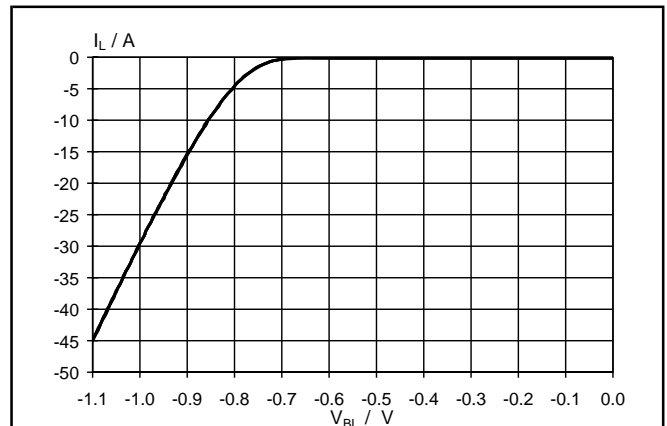
Fig.26. Typical reverse diode characteristic. I_L = f(V_{BL}) ; conditions V_{IG} = 0\text{V} , T_j = 25\text{ }^{\circ}\text{C}
