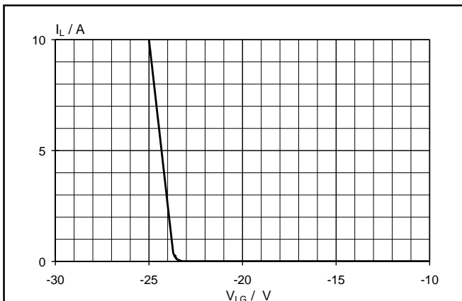
Fig.24. Typical negative load clamping. I_L = f(V_{LG}) ; conditions V_{IG} = 0\text{V} , T_j = 25\text{ }^{\circ}\text{C}
