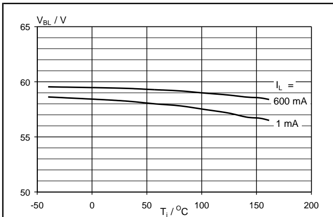
Fig.23. Typical battery to load clamping voltage. V_{BL} = f(T_j) ; parameter I_L ; condition I_G = 10\text{mA}
