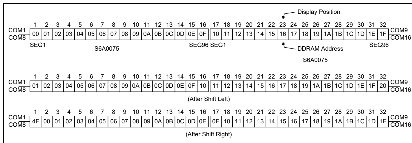
Figure 5. 1-line x 32ch. Display
