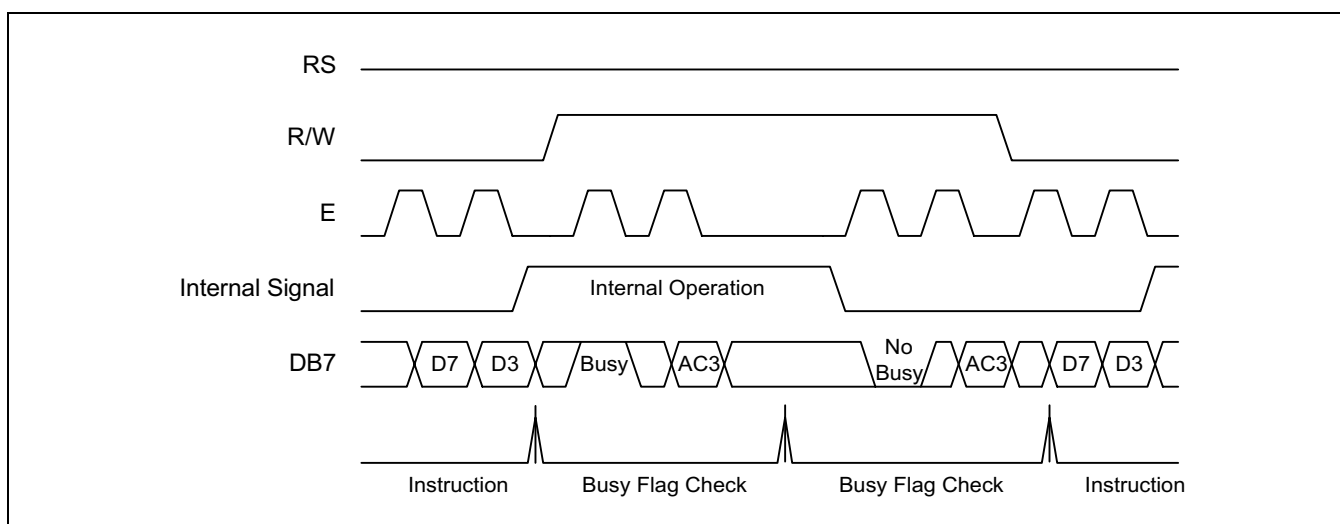
Figure 12. Example of 4-bit Bus Mode Timing Sequence
