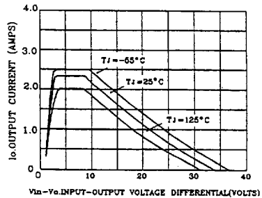
FIGURE 6 - PEAK OUTPUT CURRENT AS A FUNCTION OF INPUT-OUTPUT DIFFERENTIAL VOLTAGE
