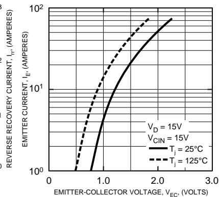
DIODE FORWARD CHARACTERISTICS
