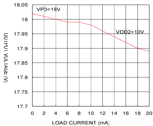
POWER 3 OUTPUT VOLTAGE VS. LOAD CURRENT
