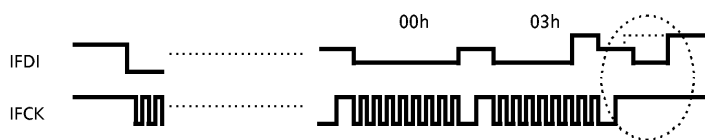
Fig.5 Timing at the Time of Self Boot Command Transmission
