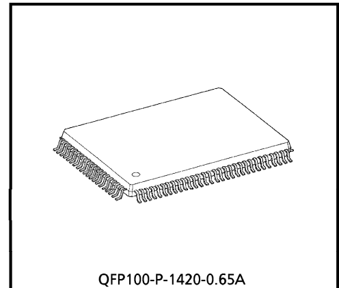
QFP100-P-1420-0.65A Weight : 1.57g (Typ.)
