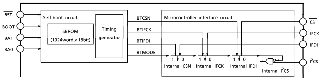
Fig.1 Self-Boot System
