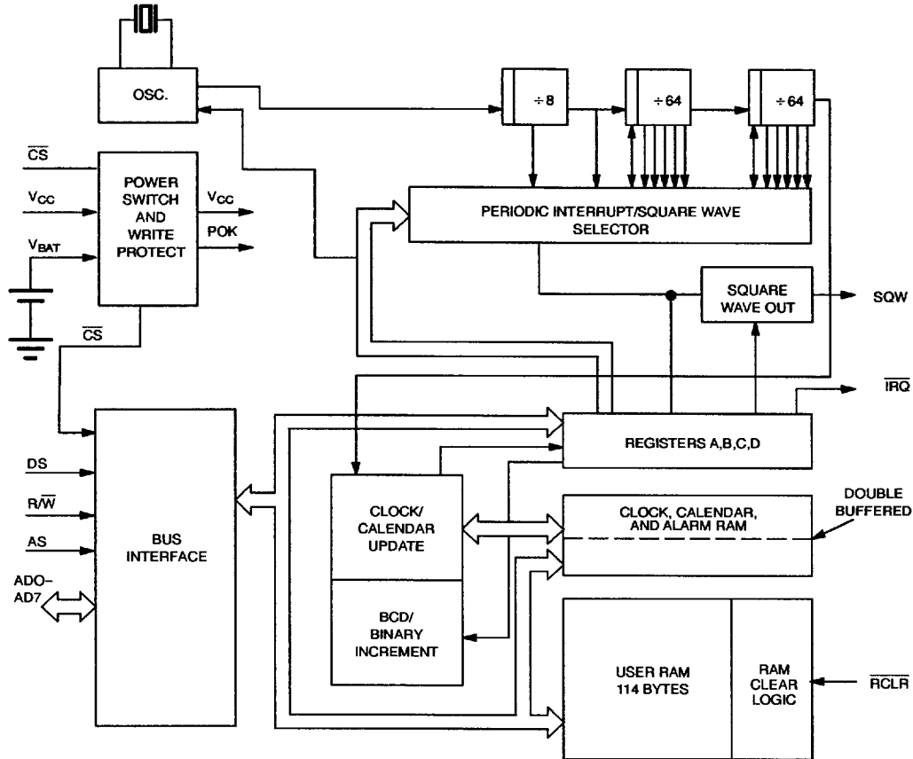
BLOCK DIAGRAM DS12B887 Figure 1
