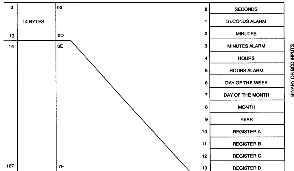
ADDRESS MAP DS12B887 Figure 2
