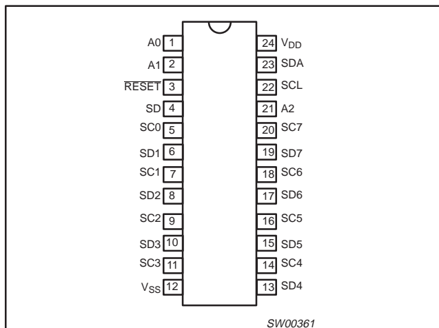
Figure 1. Pin configuration
