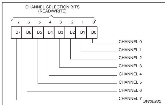
Figure 4. Control register
