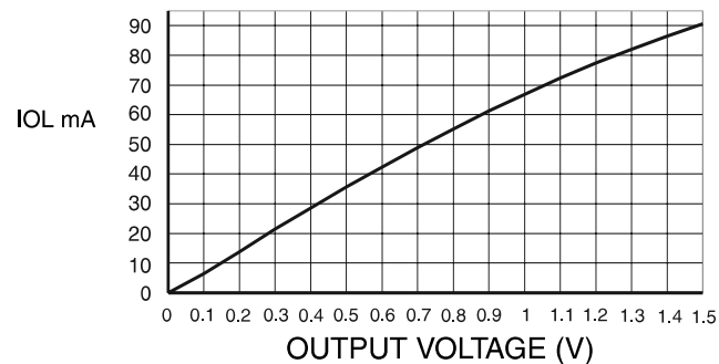
OUTPUT SINK CURRENT VS. OUTPUT VOLTAGE
