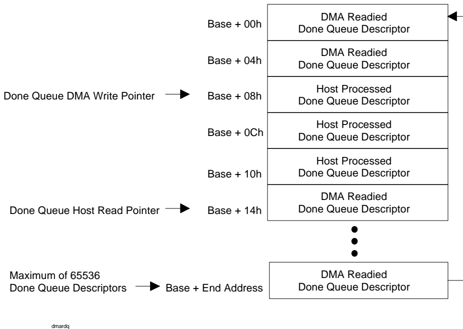
Receive Done Queue Structure Figure 8.1.4B
