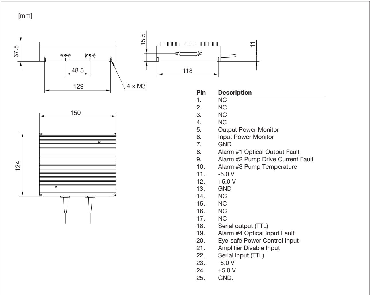
Figure 2. Mechanical outline and pin description
