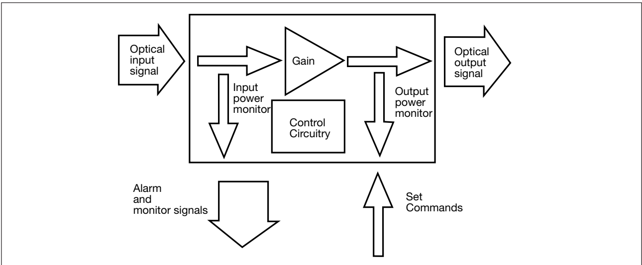
Figure 1. Block diagram
