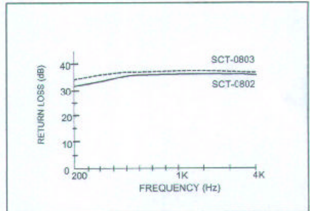
RETURN LOSS VS FREQUENCY CURVE:
