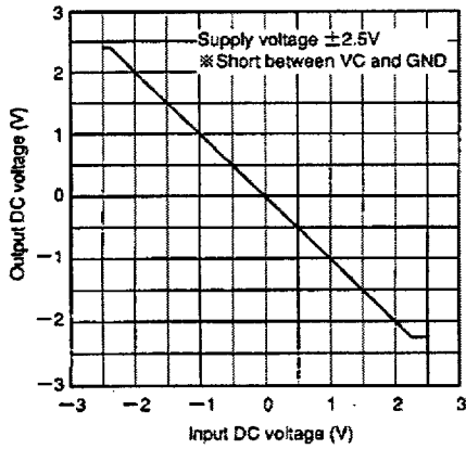
FE adjustment range characteristics
