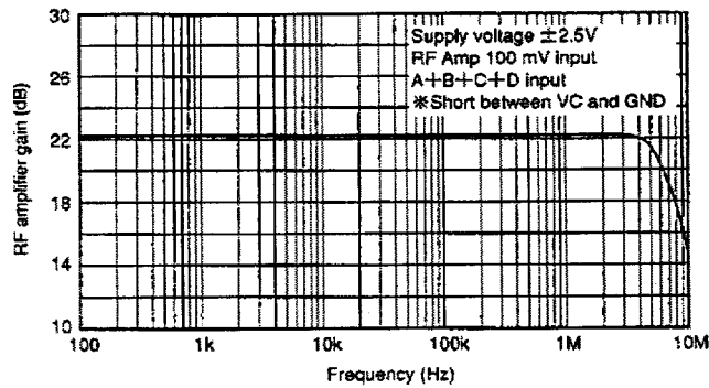
RF amplifier frequency characteristics
