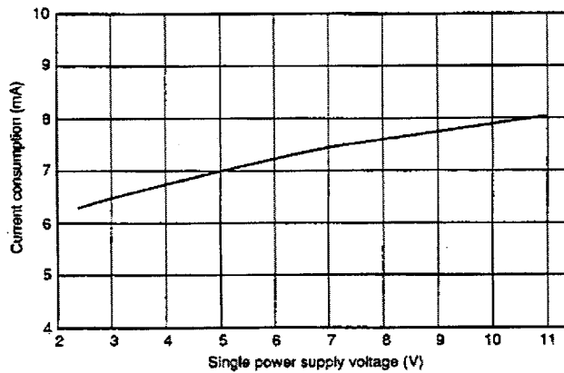
Current consumption characteristics
