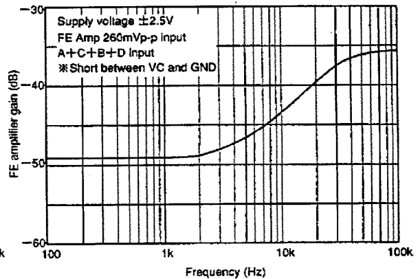
FE amplifier frequency error characteristics
