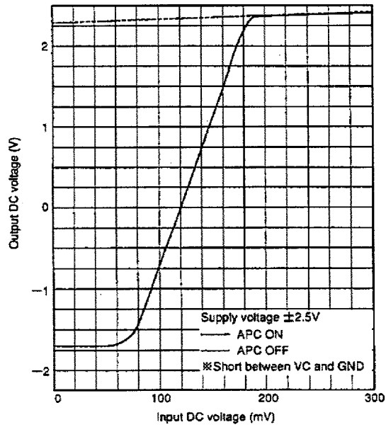
APC I/O voltage characteristics
