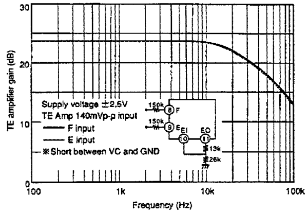
TE amplifier frequency error characteristics
