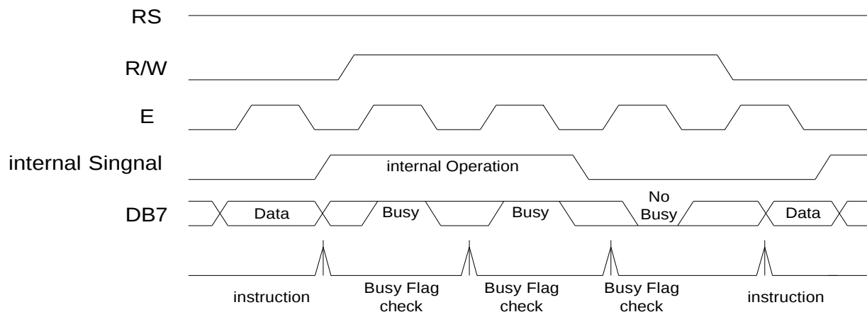
Figure 5.0 Example or 8-bit bus mode timing Diagram
