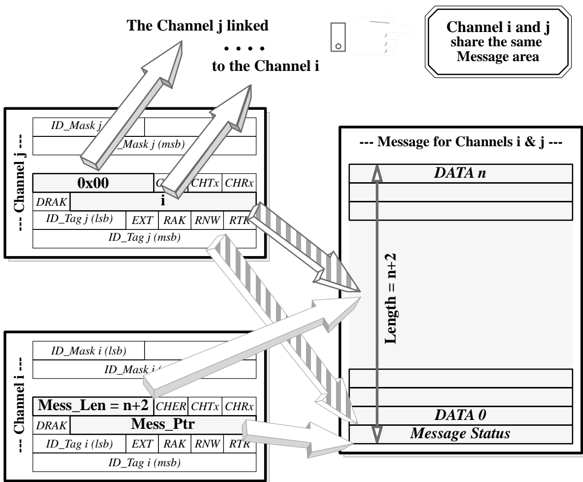
Figure 31. Linkage mechanism
