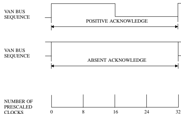
Figure 12. Acknowledge Sequences.
