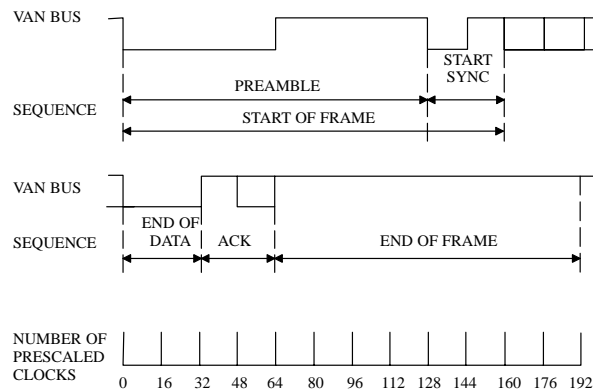
Figure 10. Framing Sequences.
