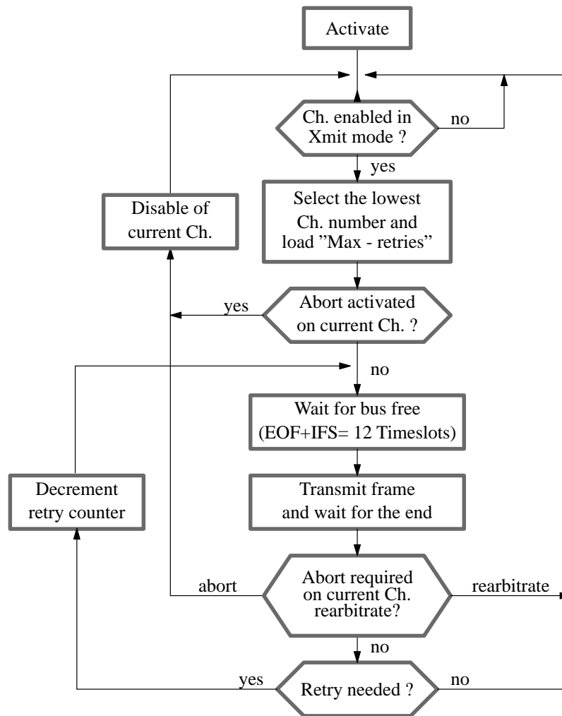
Figure 25. Transmit function
