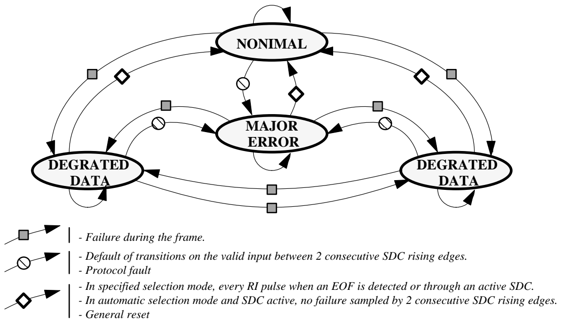
Figure 17. Diagnosis States
