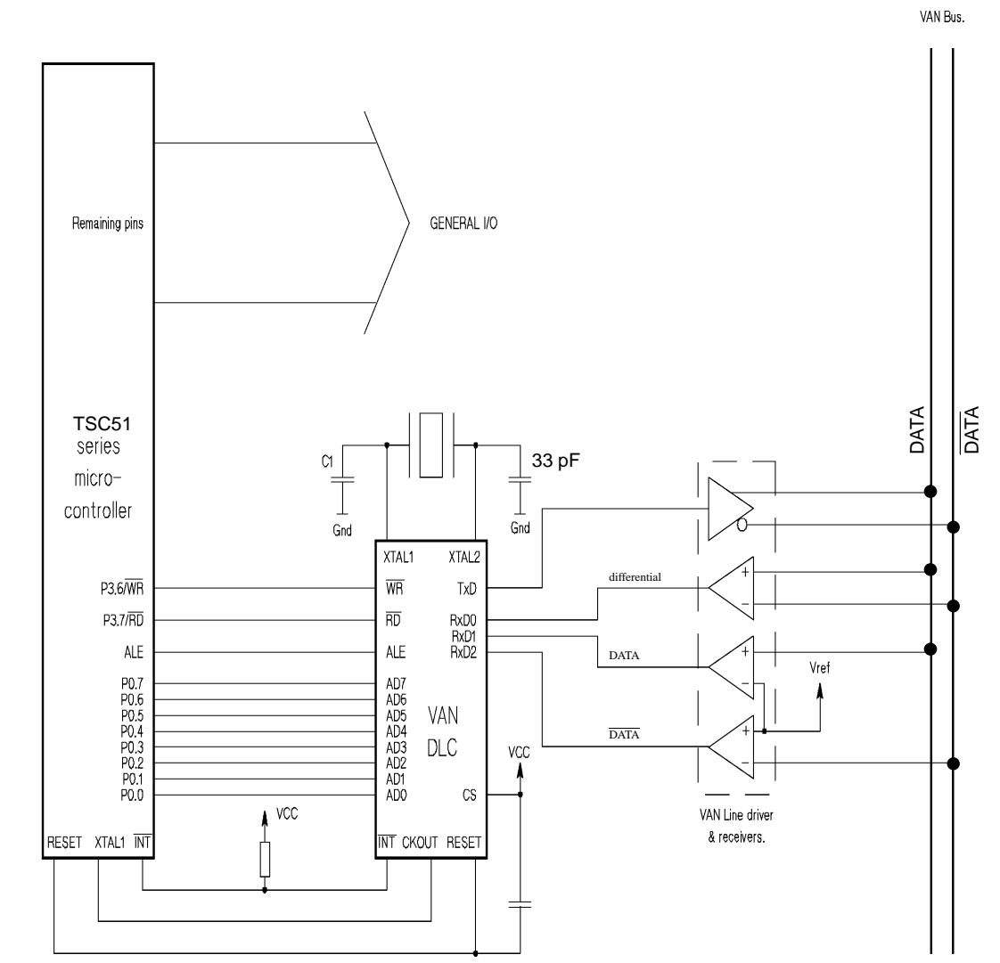
Figure 3. Typical Application
