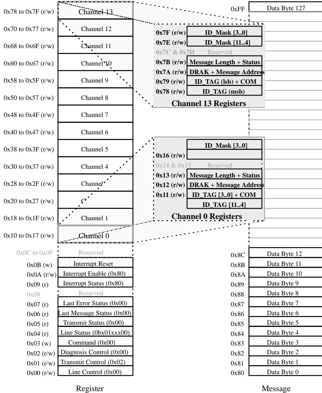
Figure 16. Memory Map.
