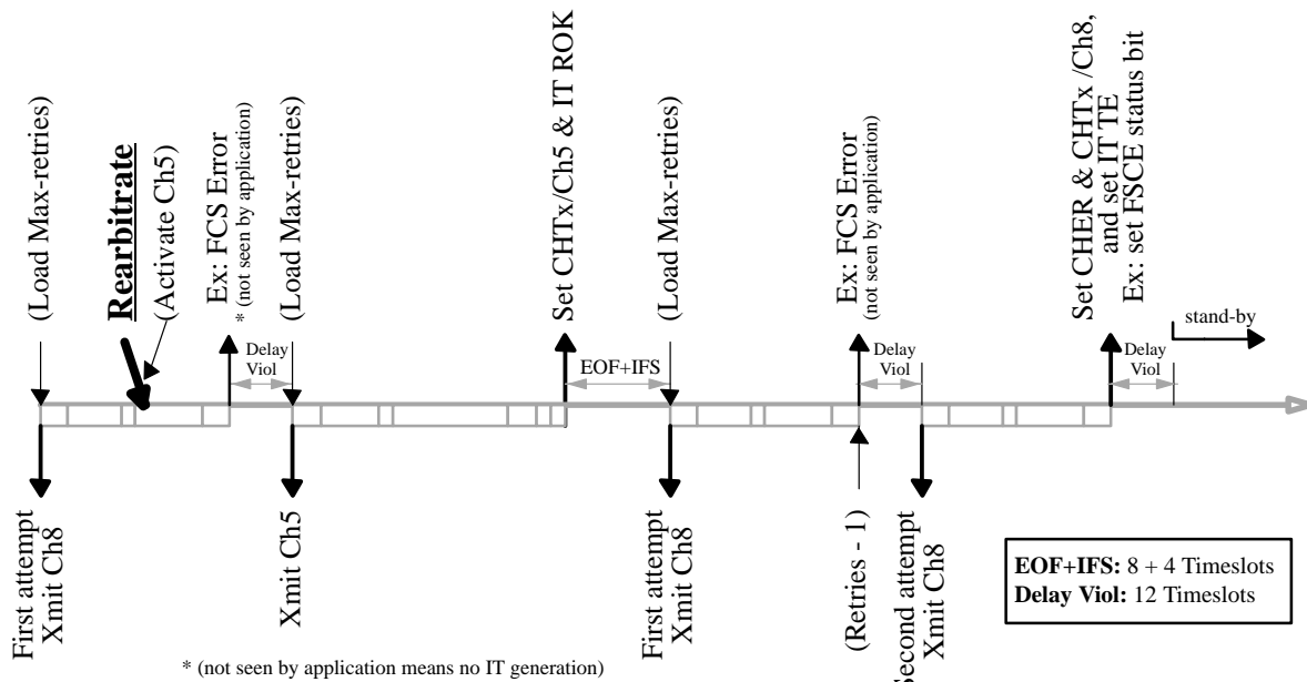
Figure 26. Rearbitrate Example
