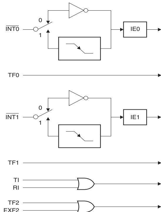
Figure 10. Interrupt Sources
