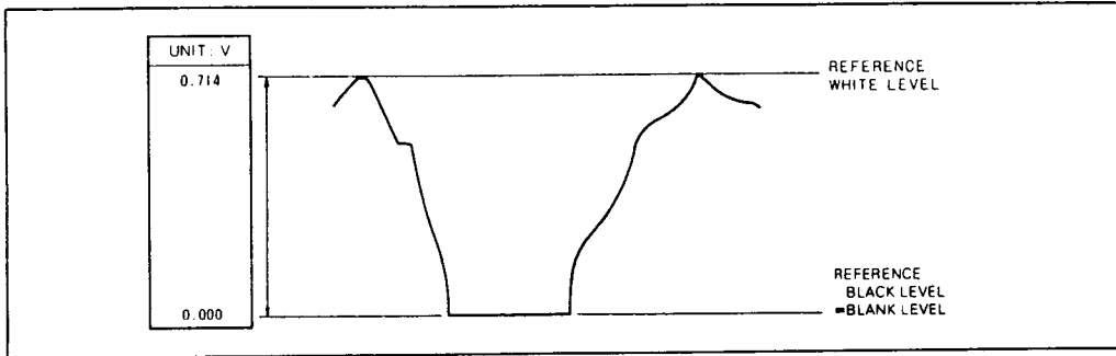
Fig. 2. (b) Video Output Waveform ( \text{BSEL} = \text{'H'} , R_{\text{REF}} = 12\text{k}\Omega )
