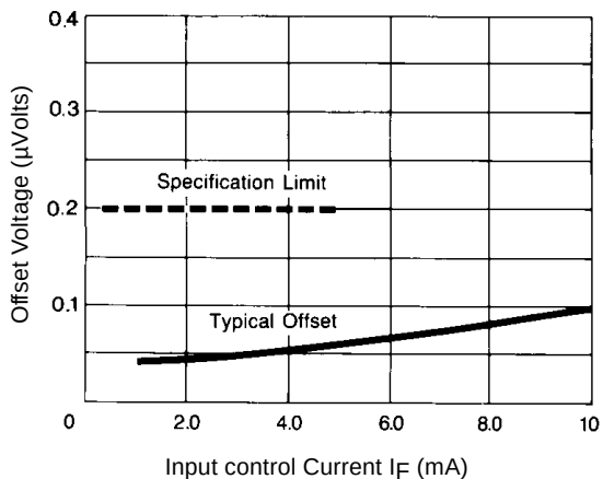
Figure 2. Offset Voltage
