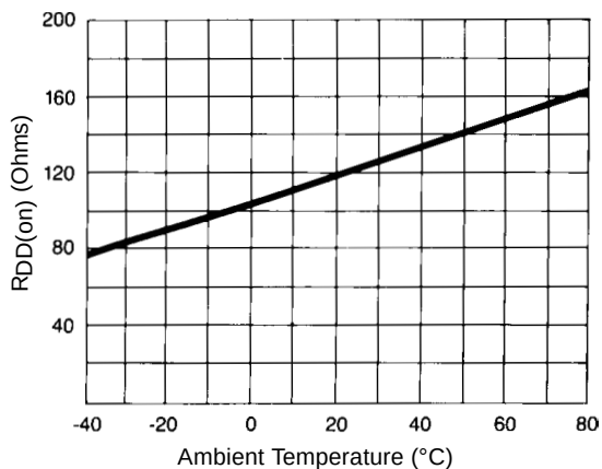
Figure 4. Typical On-Resistance
