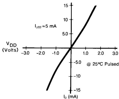
Figure 3. Typical On Characteristics
